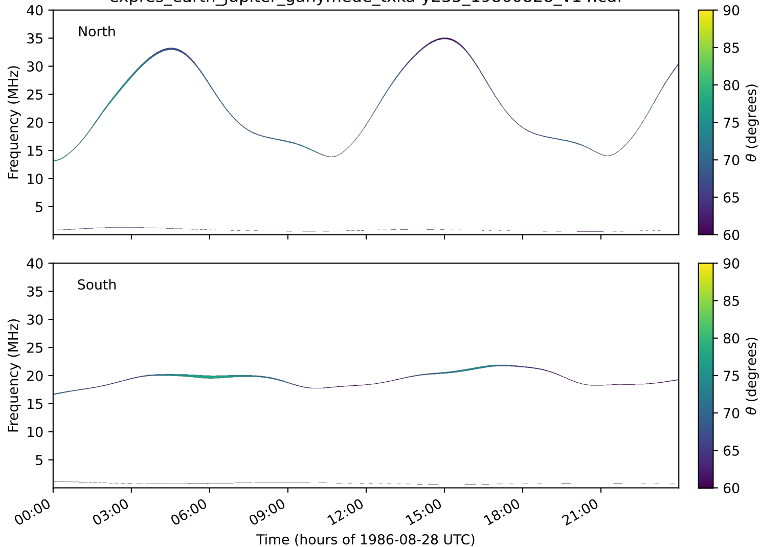
expres_earth_jupiter_ganymede_txka-y235_19860828_v14.cdf
