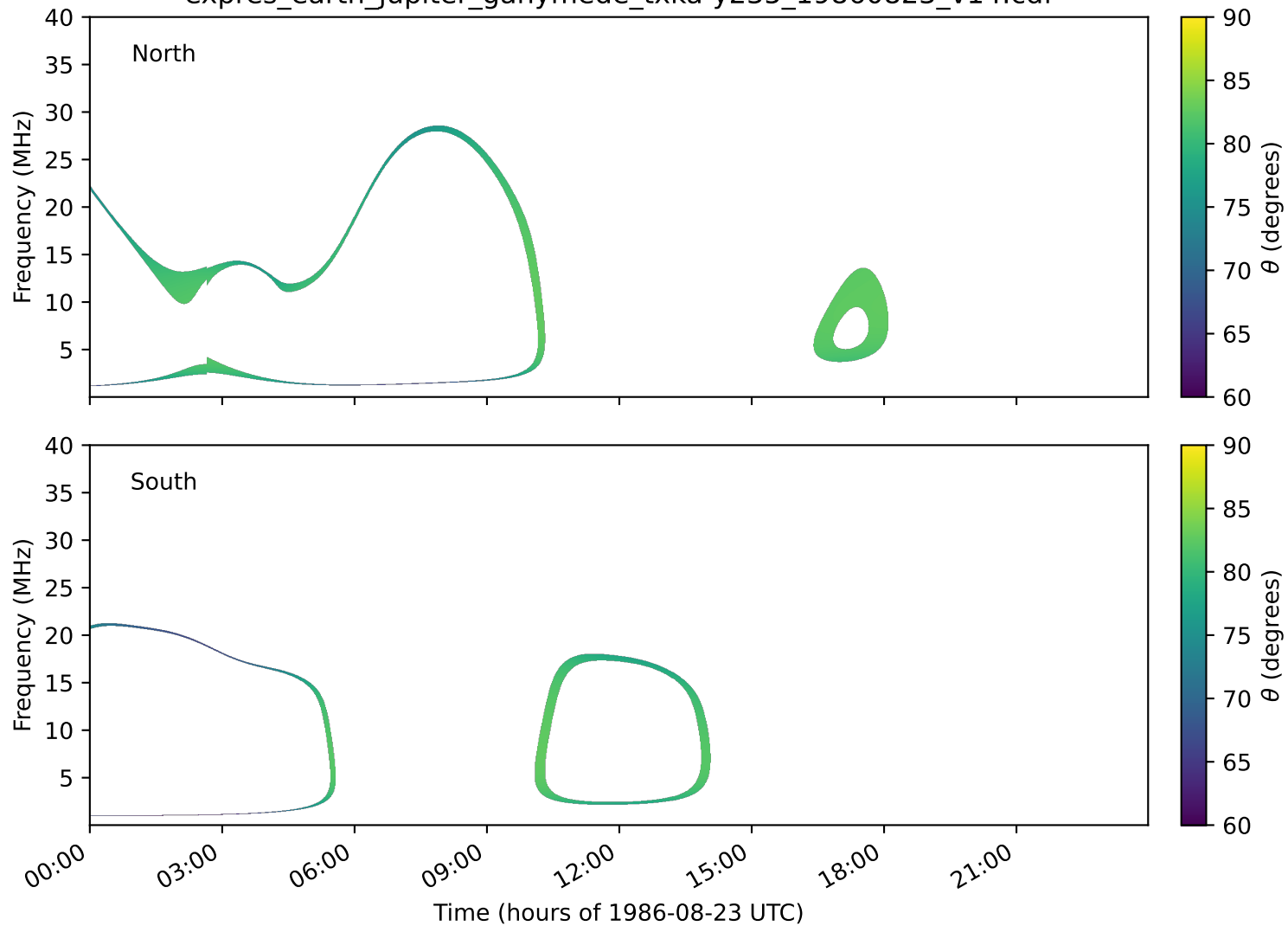
expres_earth_jupiter_ganymede_txka-y235_19860823_v14.cdf
