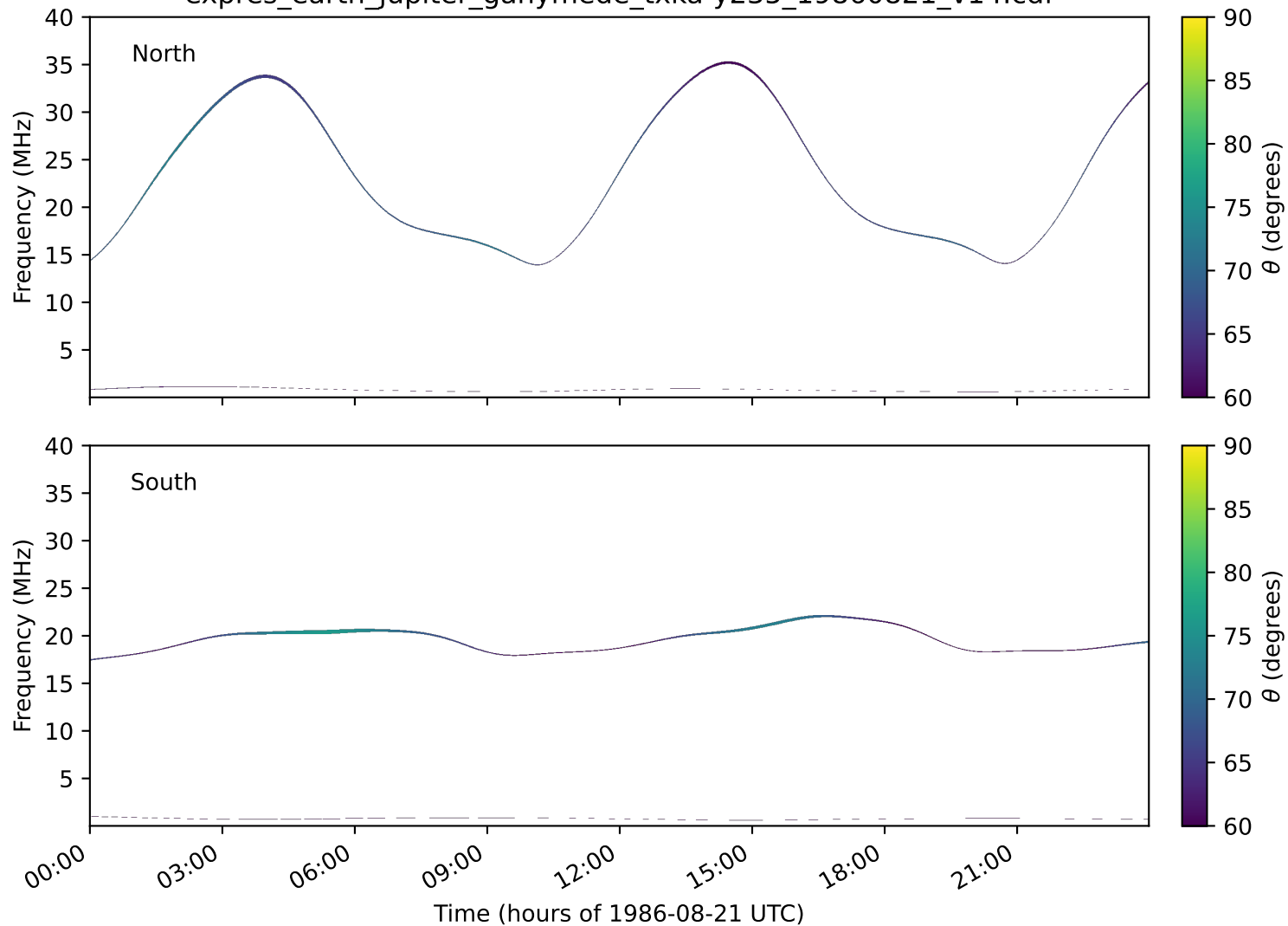
expres_earth_jupiter_ganymede_txka-y235_19860821_v14.cdf
