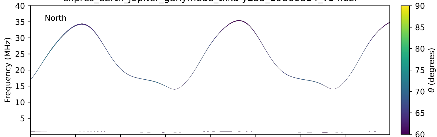
expres_earth_jupiter_ganymede_txka-y235_19860814_v14.cdf
