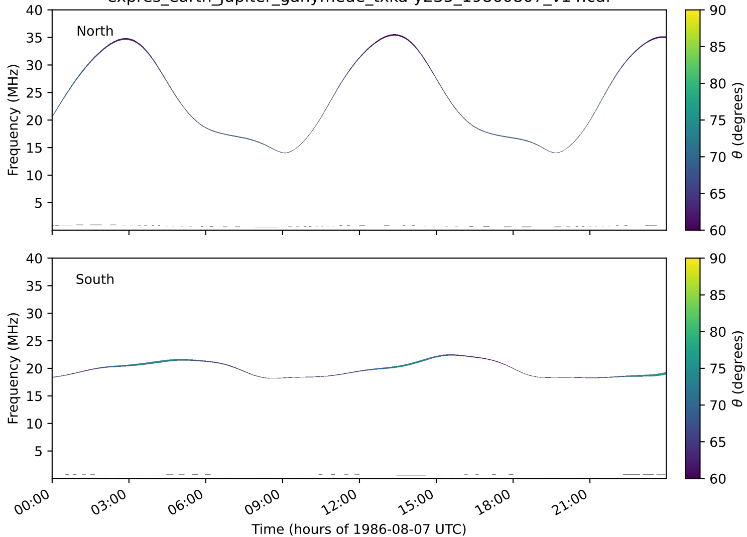
expres_earth_jupiter_ganymede_txka-y235_19860807_v14.cdf
