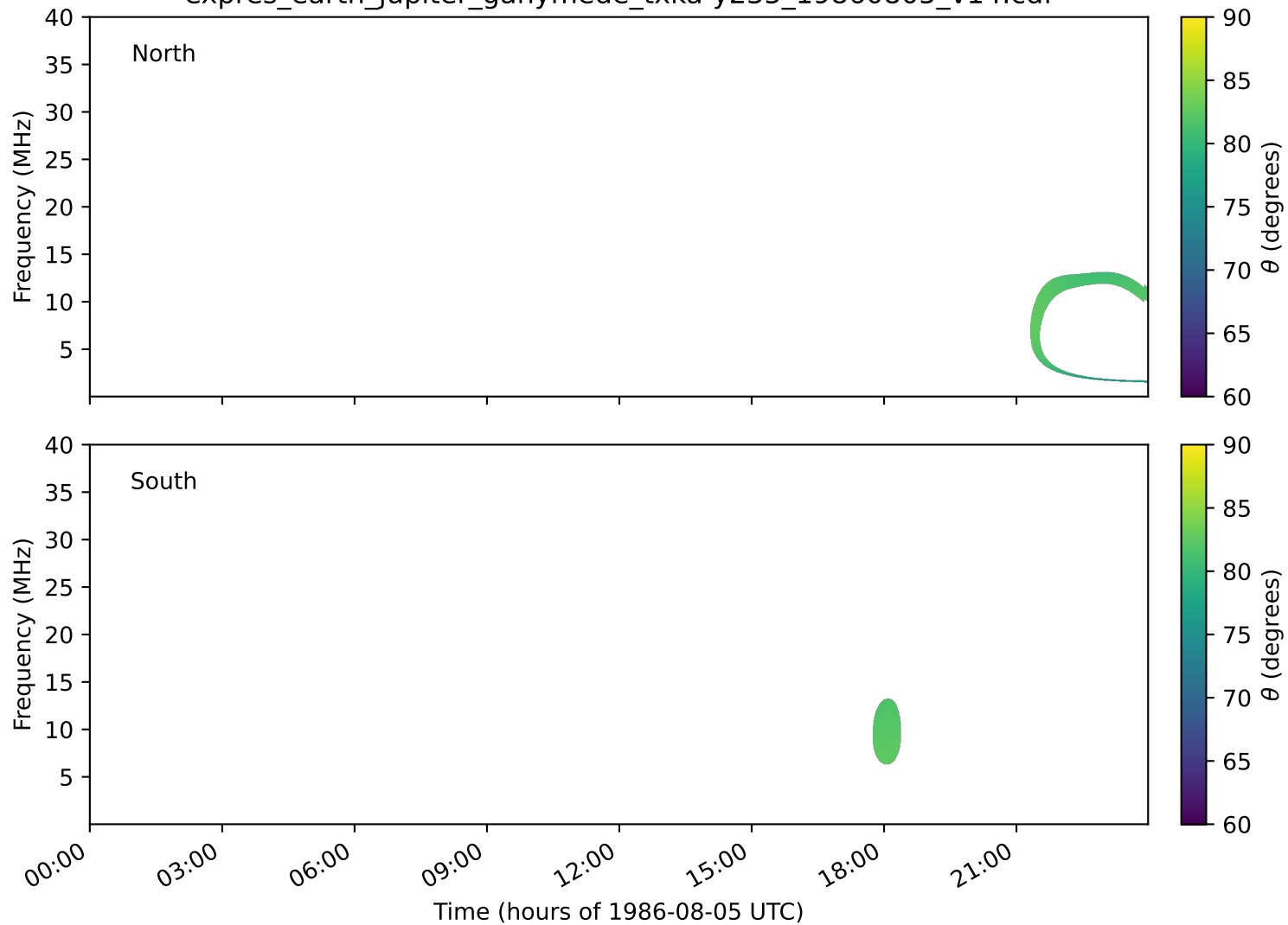
expres_earth_jupiter_ganymede_txka-y235_19860805_v14.cdf
