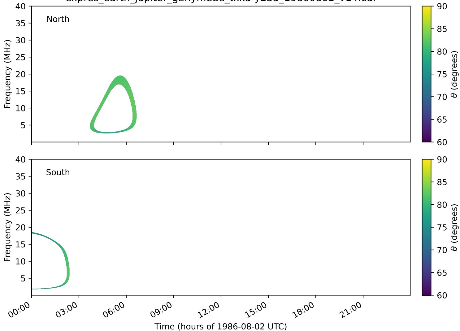
expres_earth_jupiter_ganymede_txka-y235_19860802_v14.cdf
