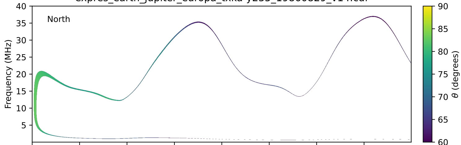
expres_earth_jupiter_europa_txka-y235_19860829_v14.cdf
