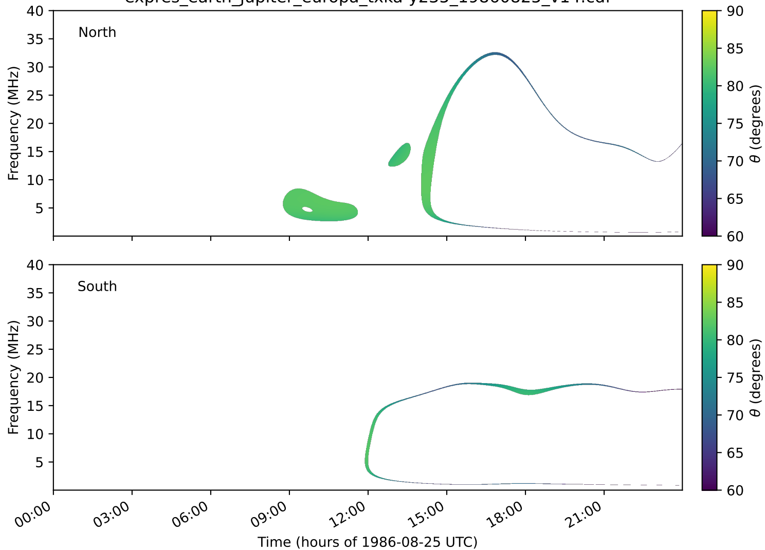
expres_earth_jupiter_europa_txka-y235_19860825_v14.cdf
