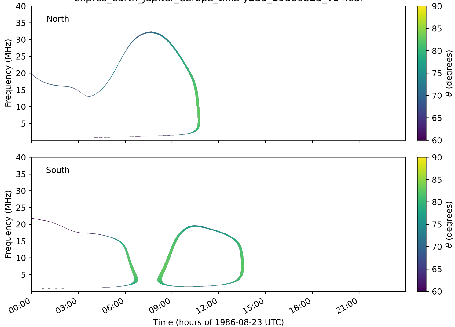
expres_earth_jupiter_europa_txka-y235_19860823_v14.cdf
