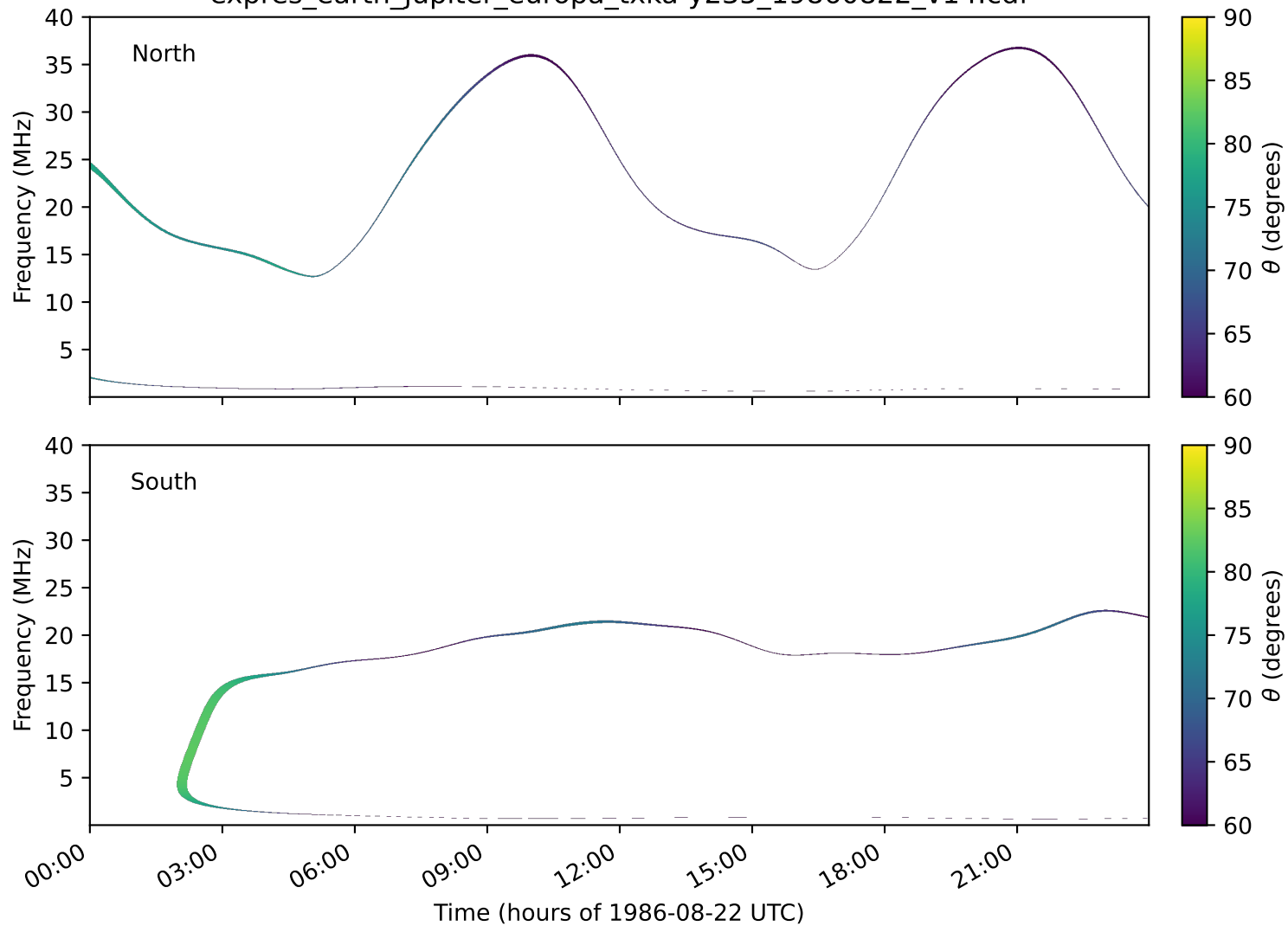
expres_earth_jupiter_europa_txka-y235_19860822_v14.cdf
