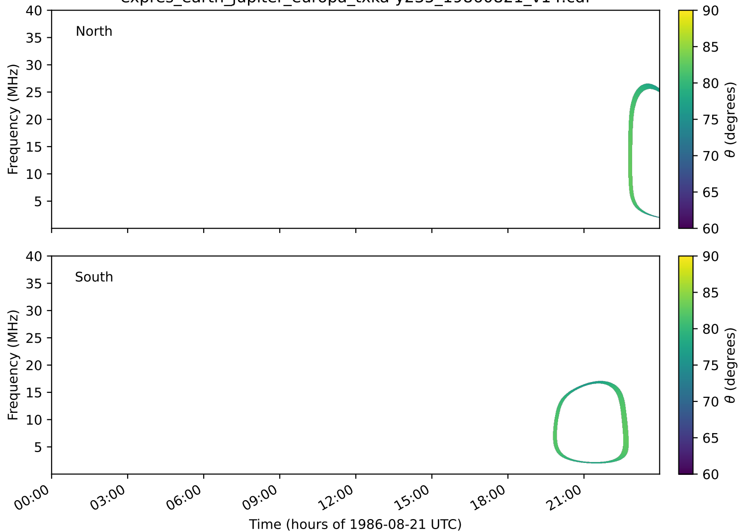
expres_earth_jupiter_europa_txka-y235_19860821_v14.cdf
