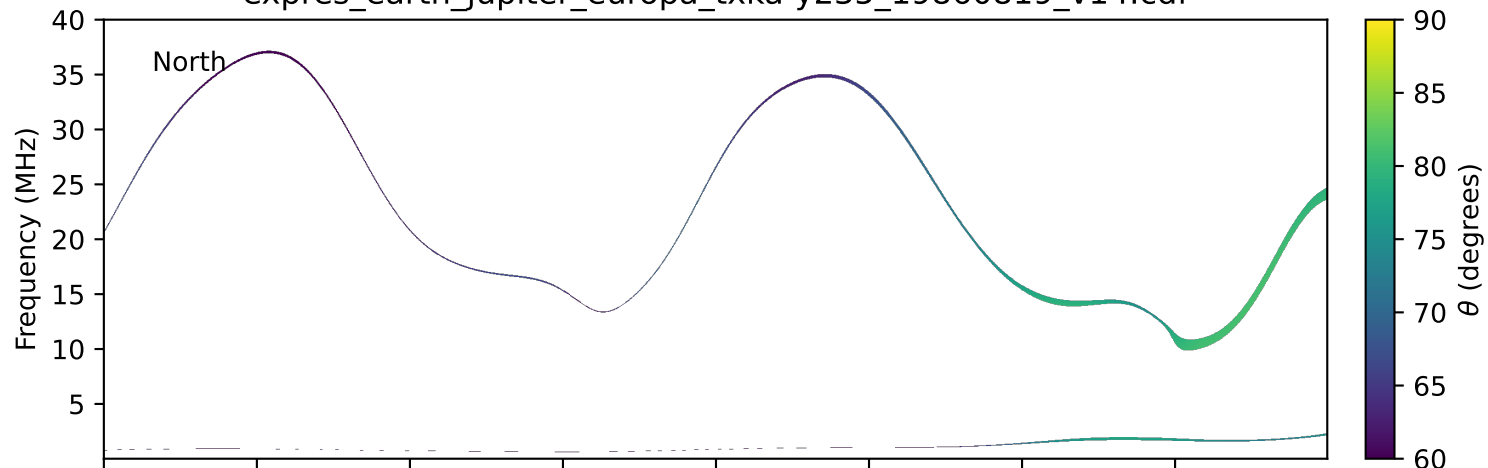
expres_earth_jupiter_europa_txka-y235_19860819_v14.cdf
