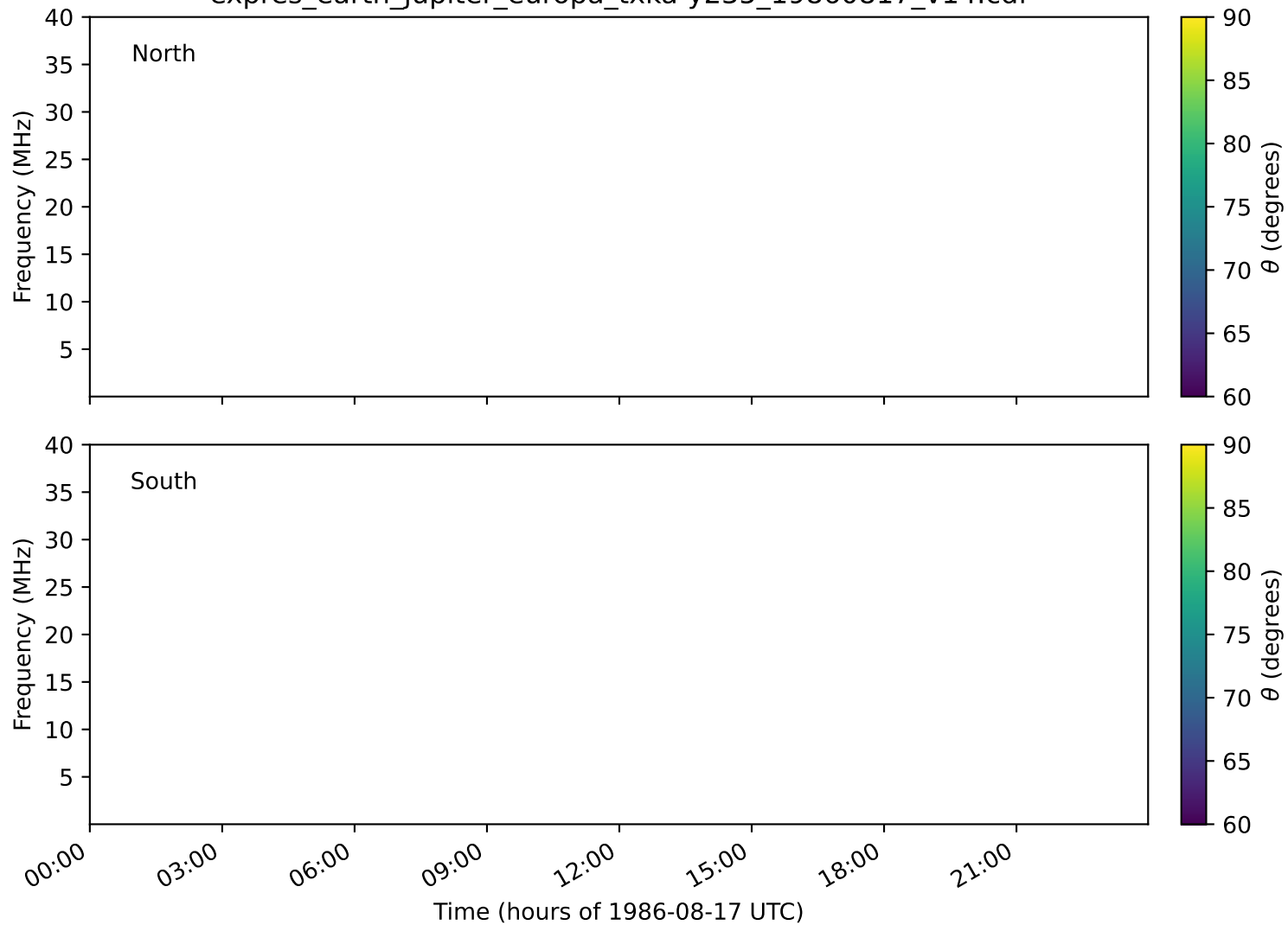
expres_earth_jupiter_europa_txka-y235_19860817_v14.cdf
