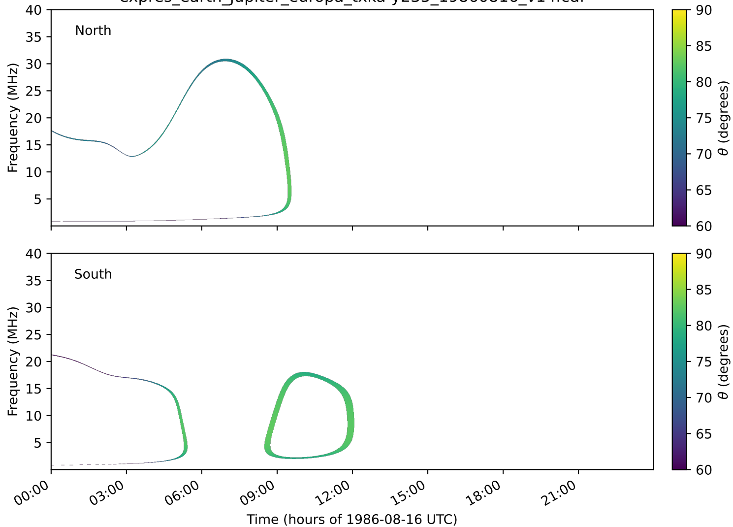
expres_earth_jupiter_europa_txka-y235_19860816_v14.cdf
