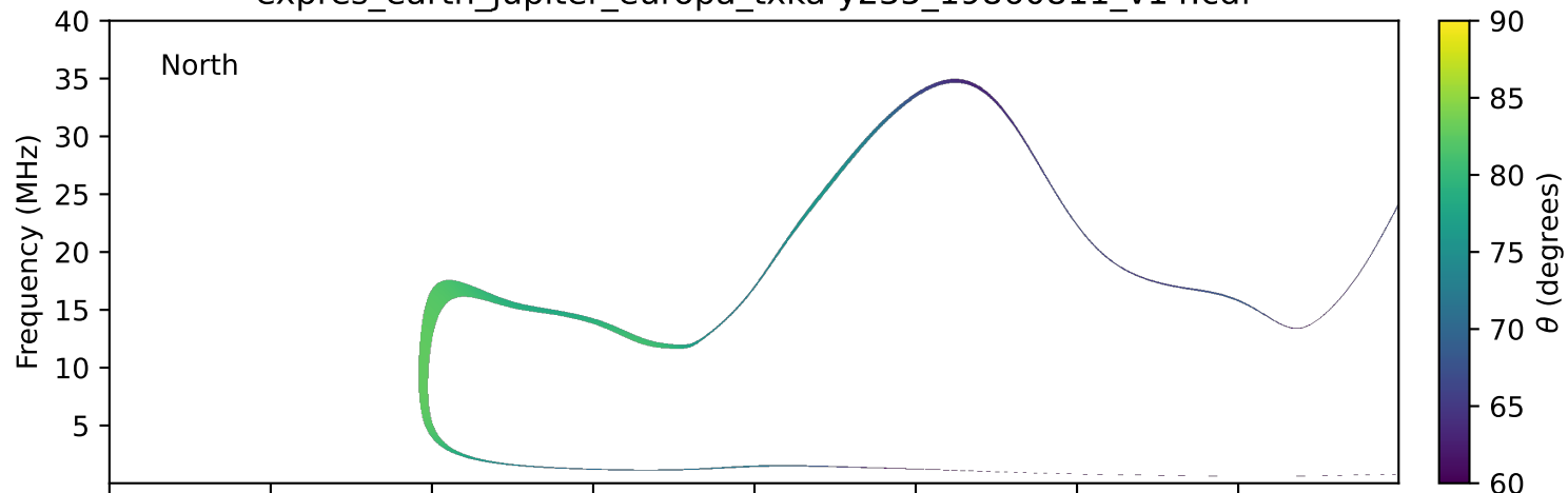
expres_earth_jupiter_europa_txka-y235_19860811_v14.cdf
