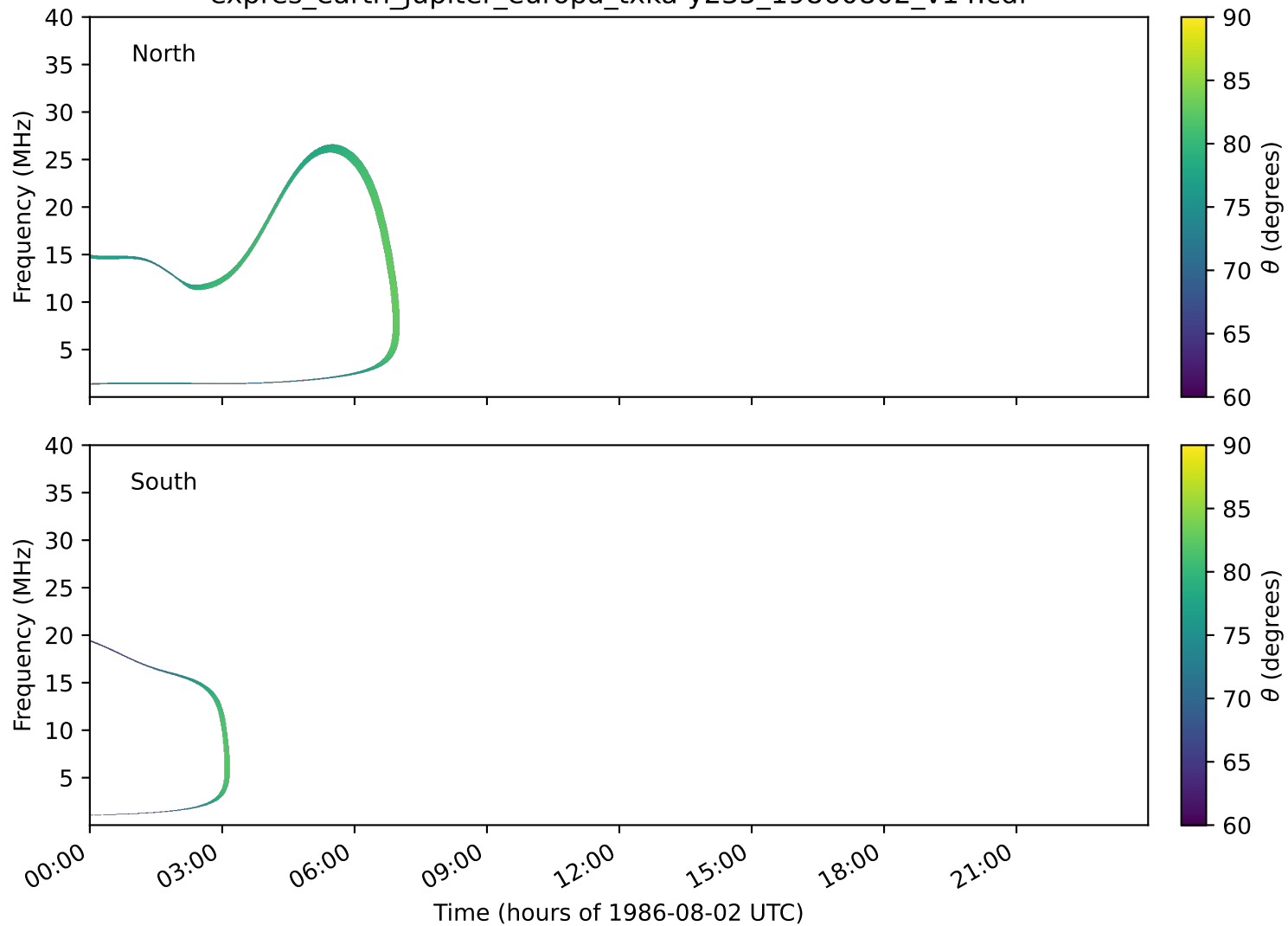
expres_earth_jupiter_europa_txka-y235_19860802_v14.cdf
