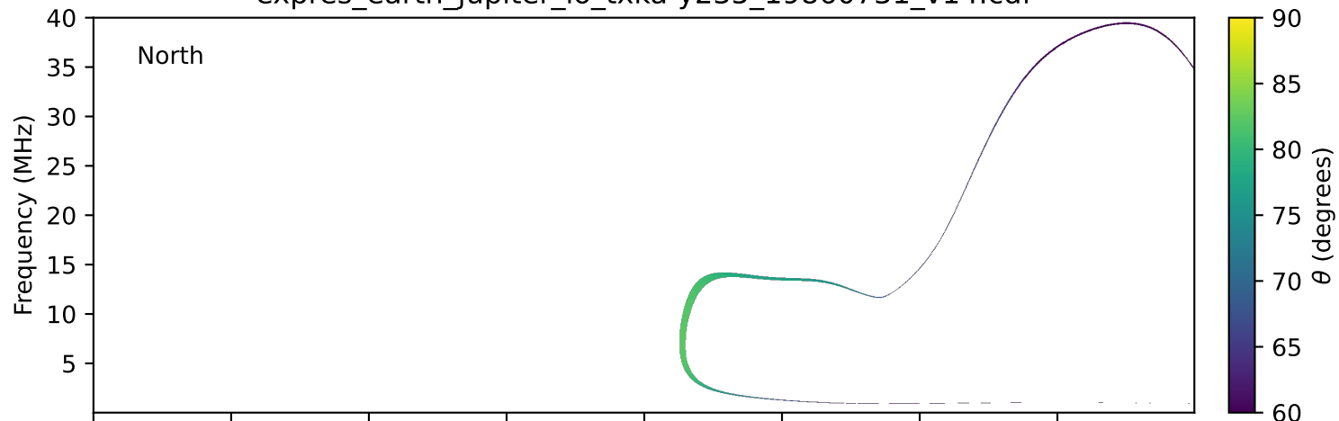
expres_earth_jupiter_io_txka-y235_19860731_v14.cdf
