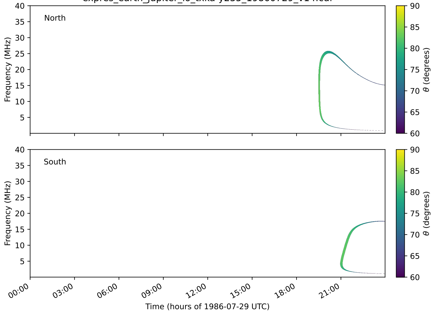
expres_earth_jupiter_io_txka-y235_19860729_v14.cdf
