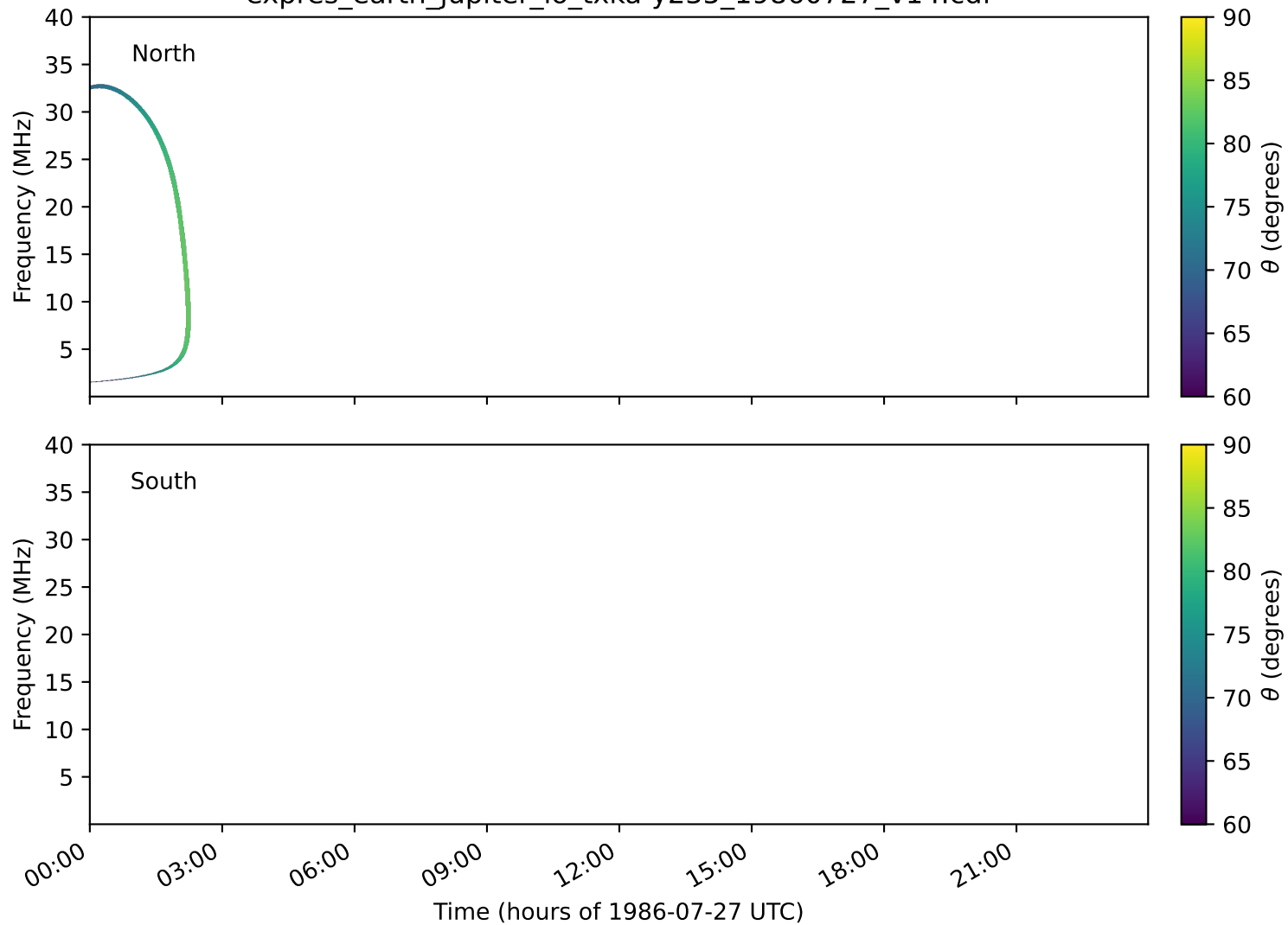
expres_earth_jupiter_io_txka-y235_19860727_v14.cdf
