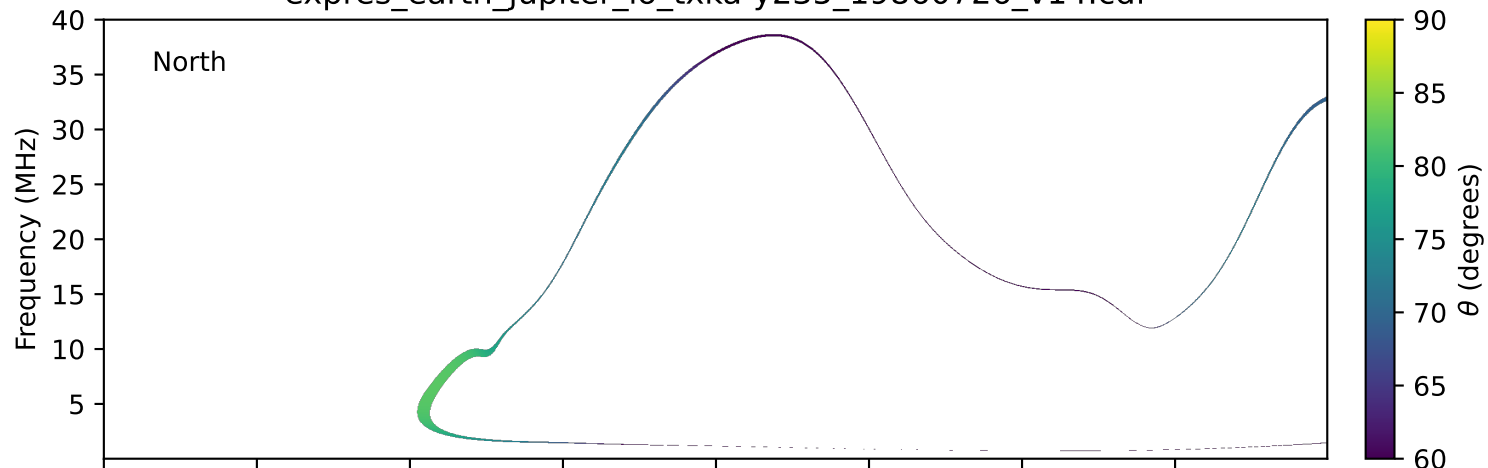
expres_earth_jupiter_io_txka-y235_19860726_v14.cdf
