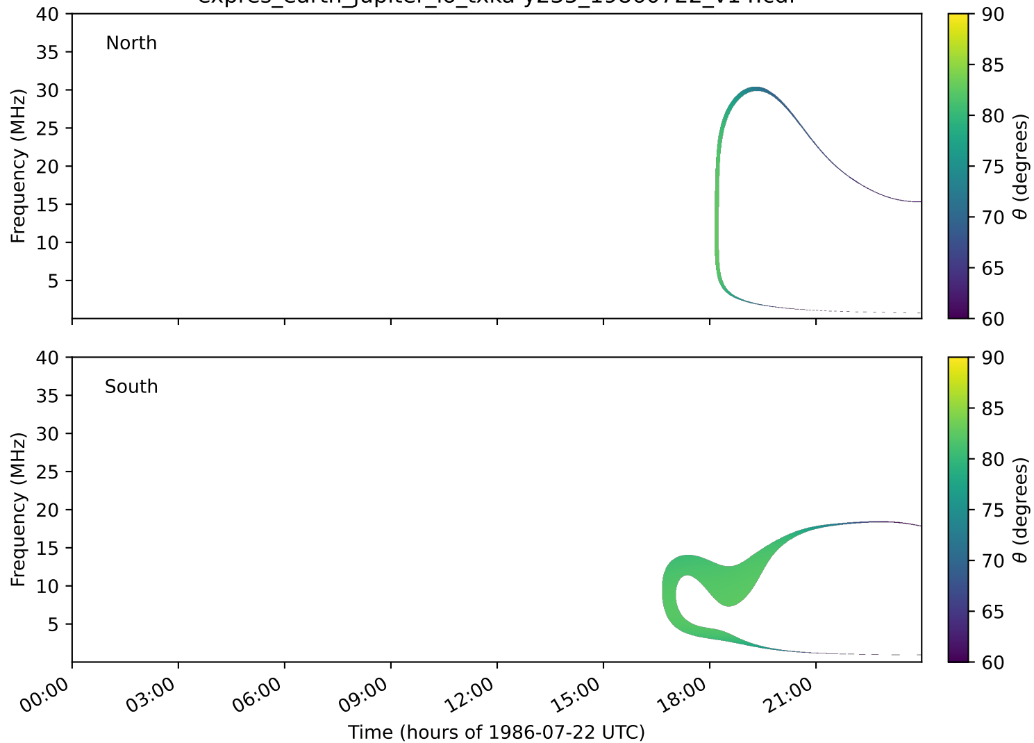
expres_earth_jupiter_io_txka-y235_19860722_v14.cdf
