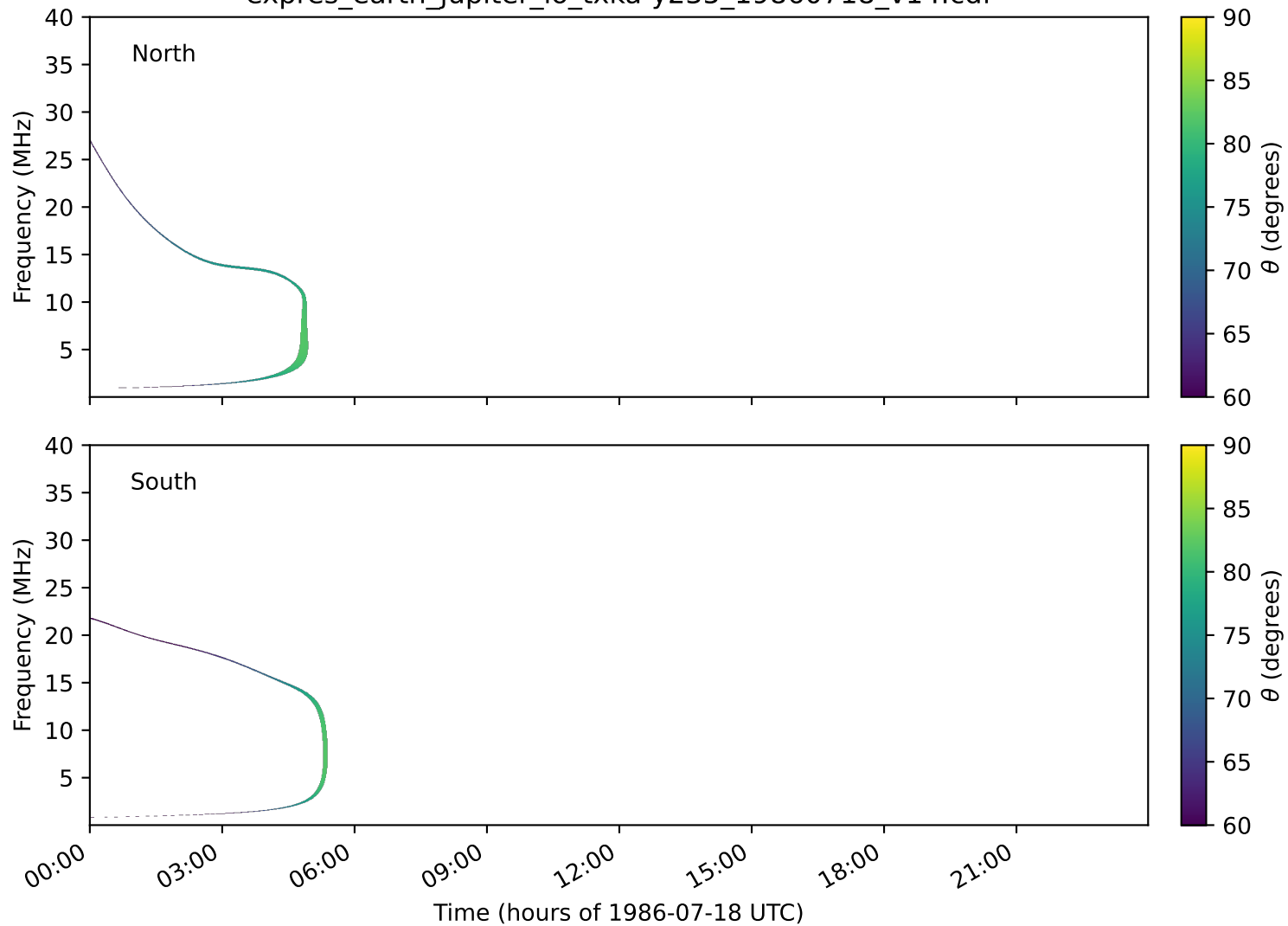
expres_earth_jupiter_io_txka-y235_19860718_v14.cdf
