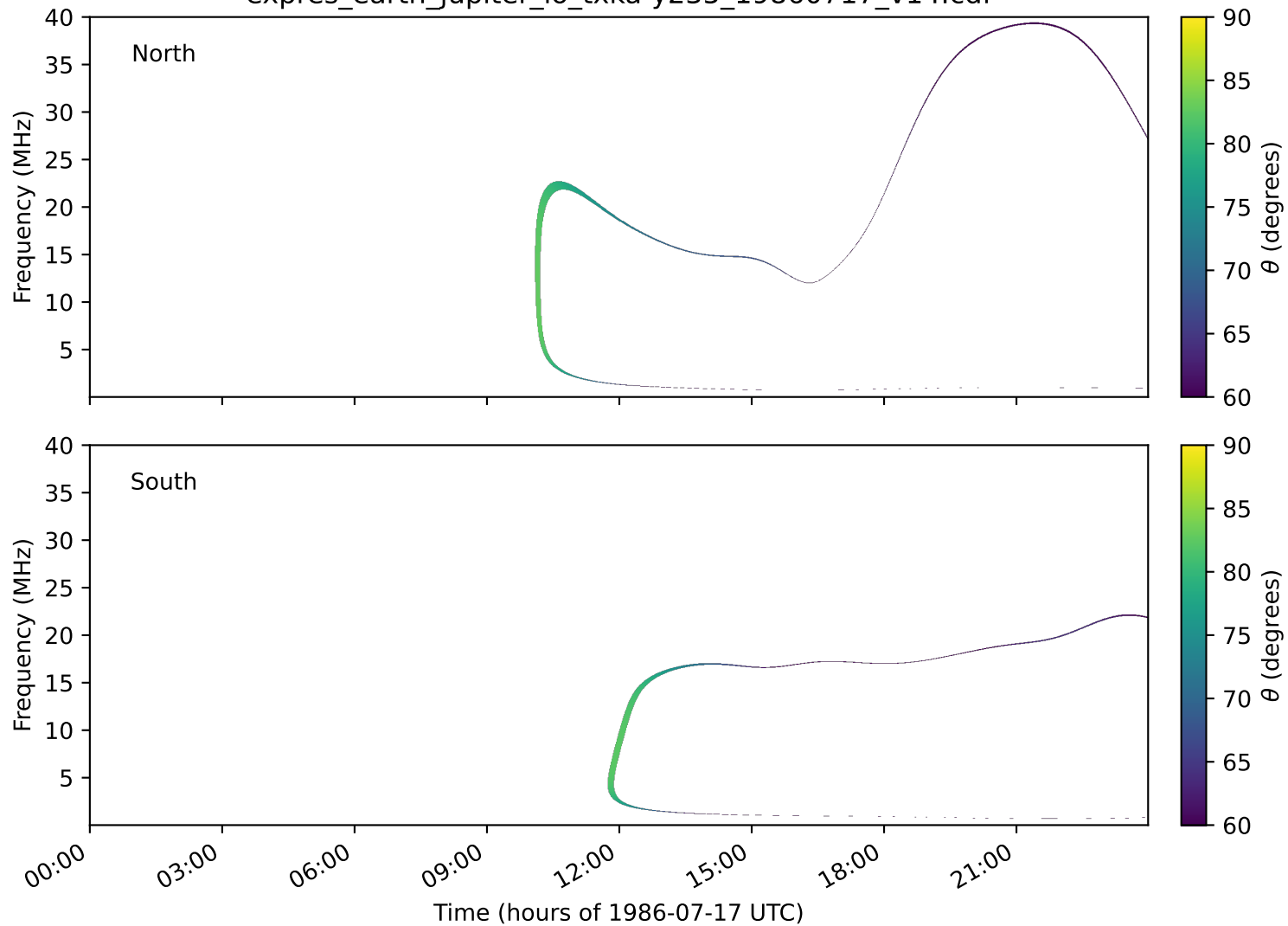
expres_earth_jupiter_io_txka-y235_19860717_v14.cdf
