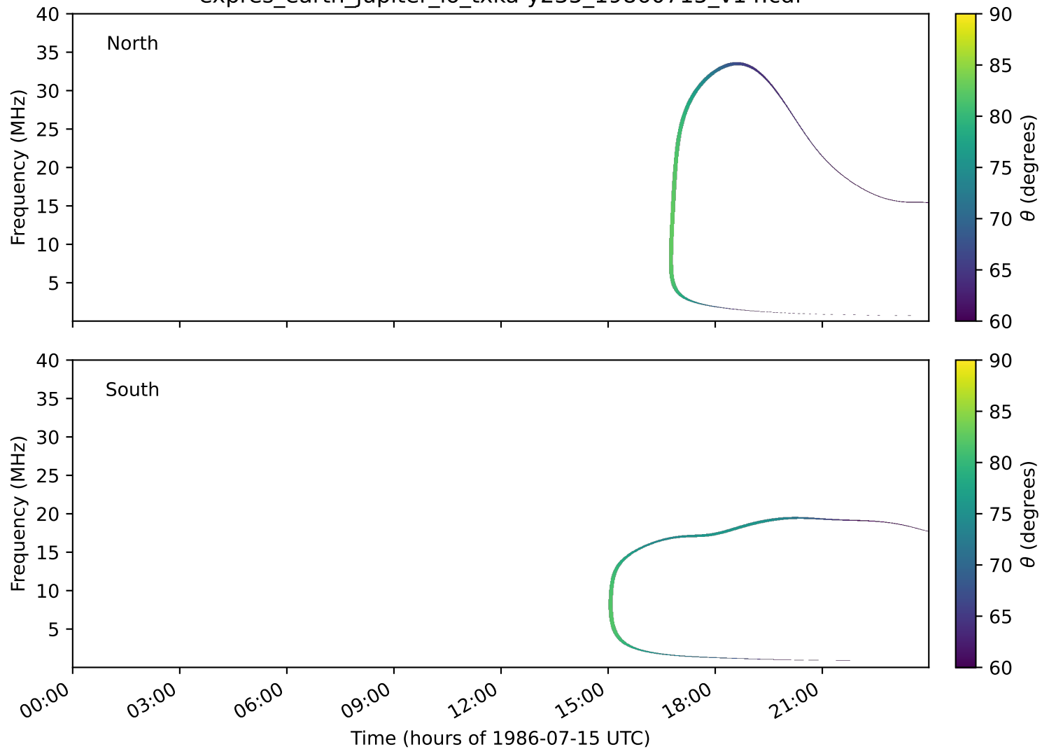
expres_earth_jupiter_io_txka-y235_19860715_v14.cdf
