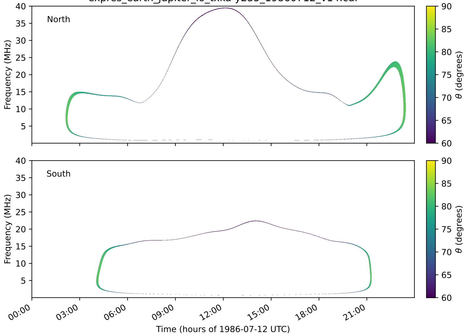
expres_earth_jupiter_io_txka-y235_19860712_v14.cdf
