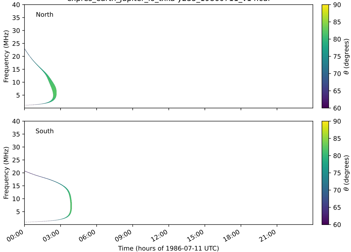
expres_earth_jupiter_io_txka-y235_19860711_v14.cdf
