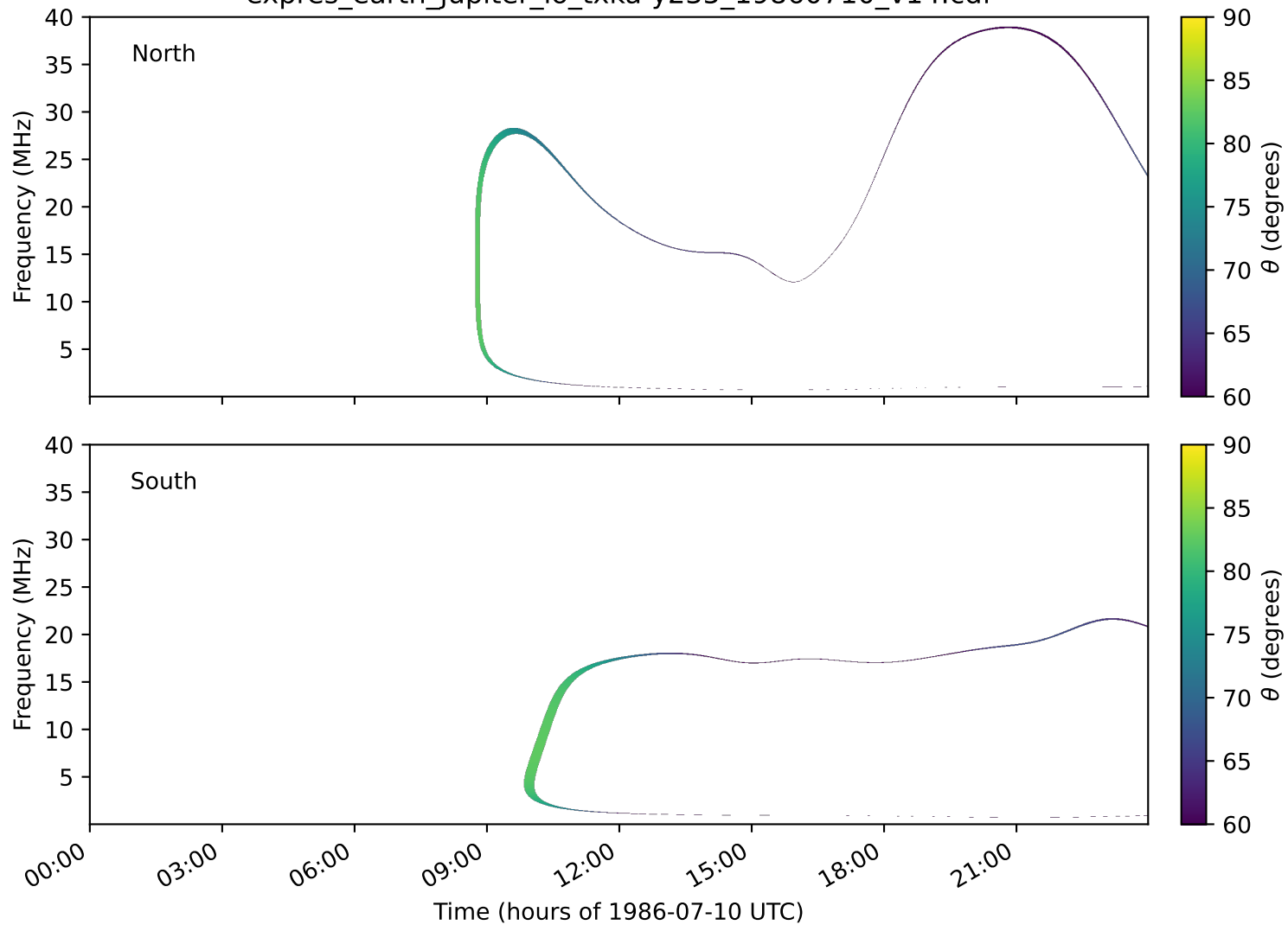
expres_earth_jupiter_io_txka-y235_19860710_v14.cdf
