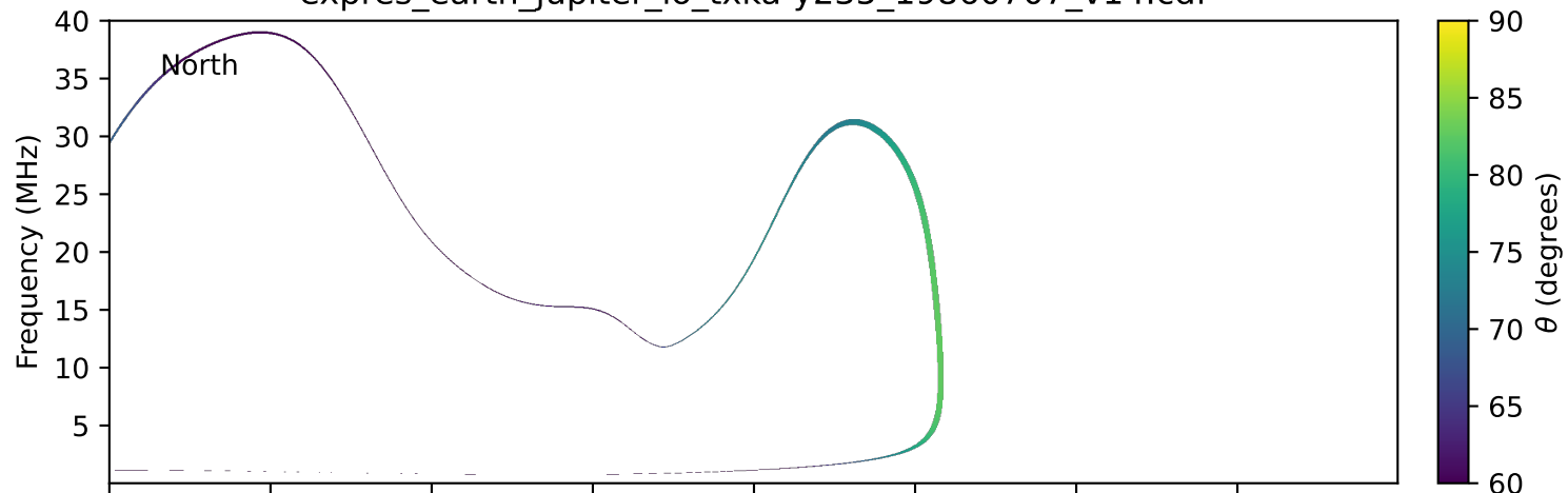
expres_earth_jupiter_io_txka-y235_19860707_v14.cdf
