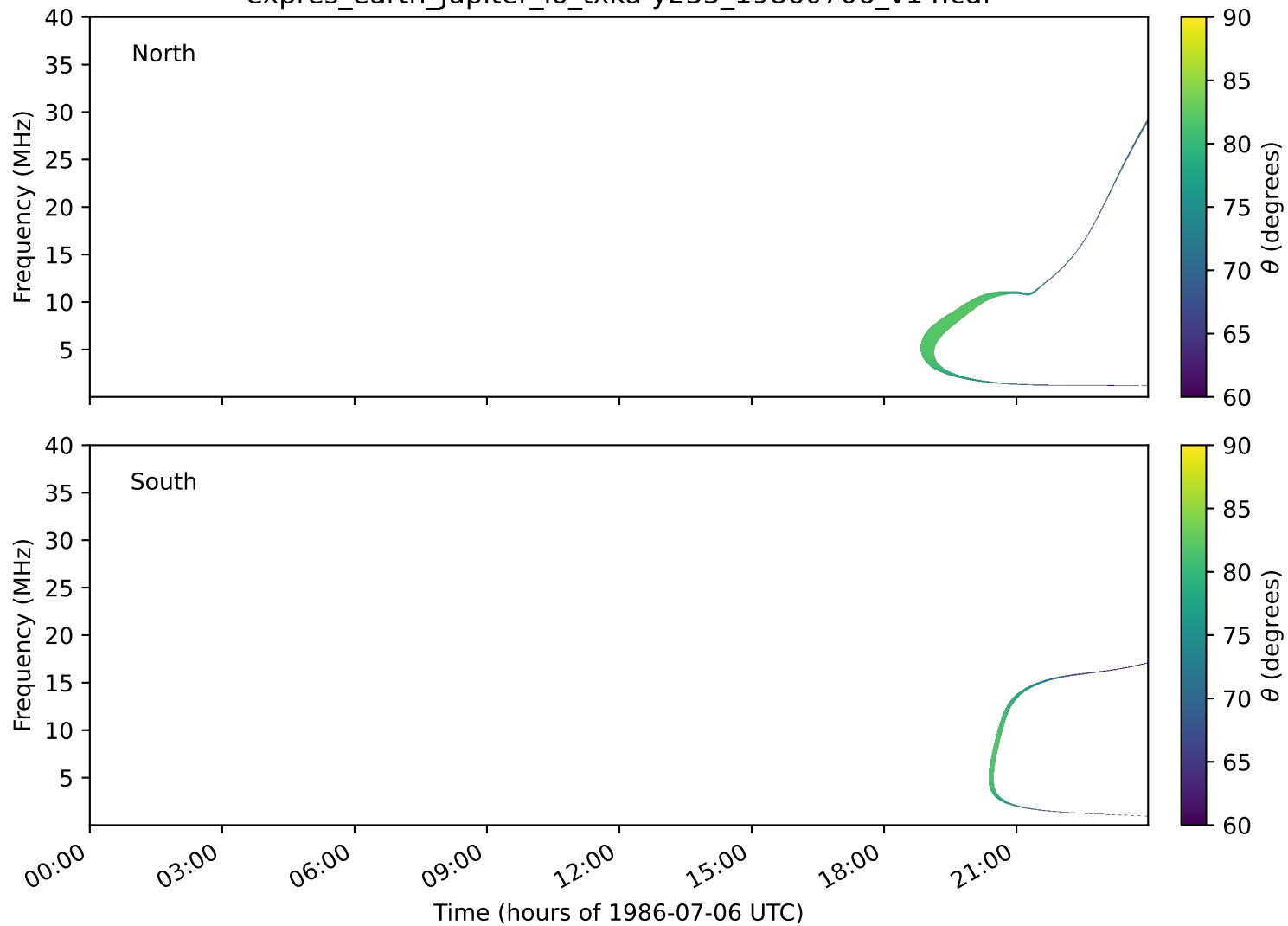
expres_earth_jupiter_io_txka-y235_19860706_v14.cdf
