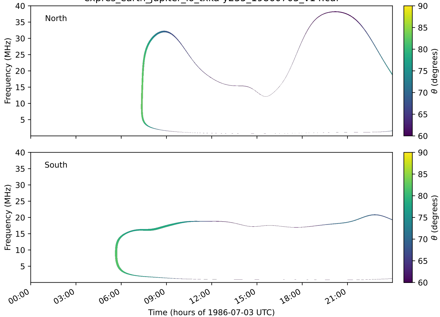
expres_earth_jupiter_io_txka-y235_19860703_v14.cdf
