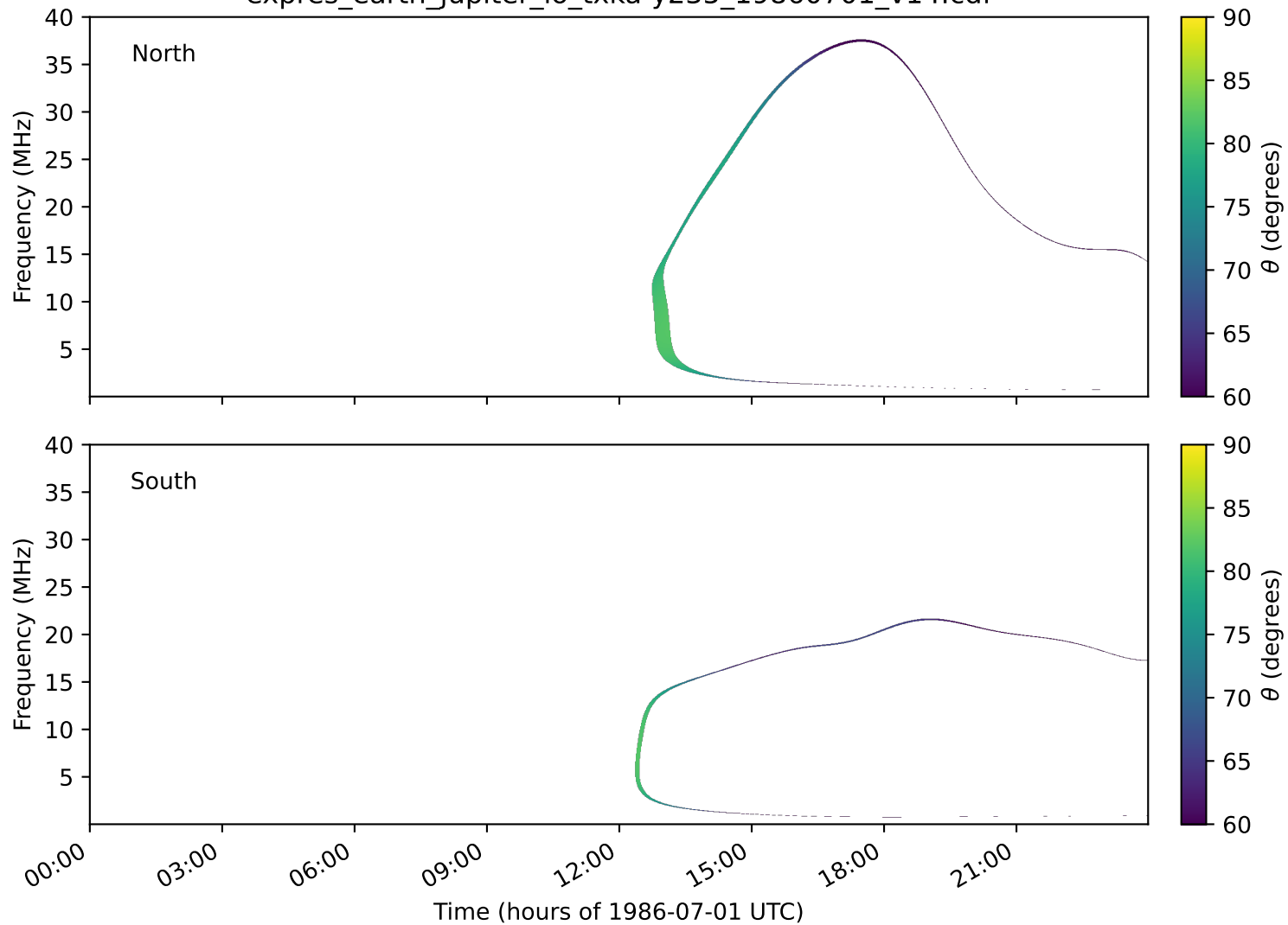
expres_earth_jupiter_io_txka-y235_19860701_v14.cdf
