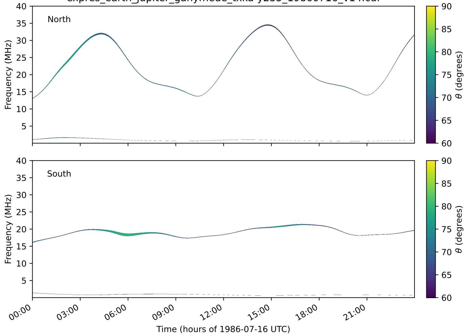
expres_earth_jupiter_ganymede_txka-y235_19860716_v14.cdf
