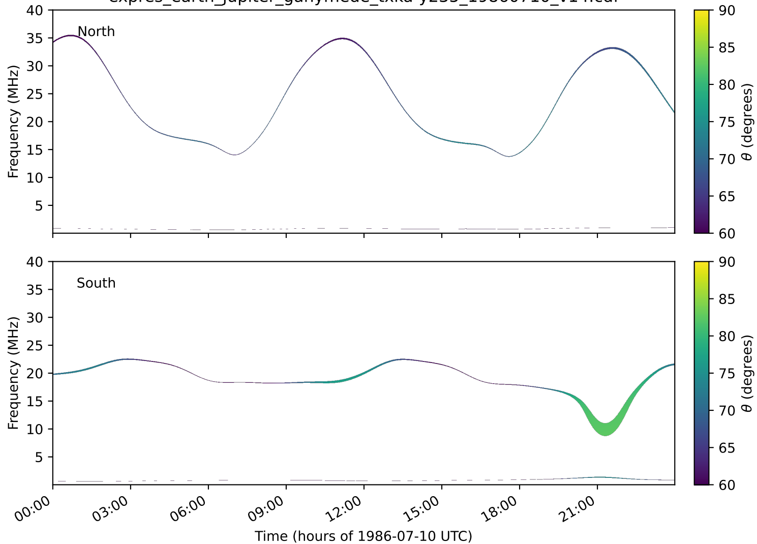
expres_earth_jupiter_ganymede_txka-y235_19860710_v14.cdf
