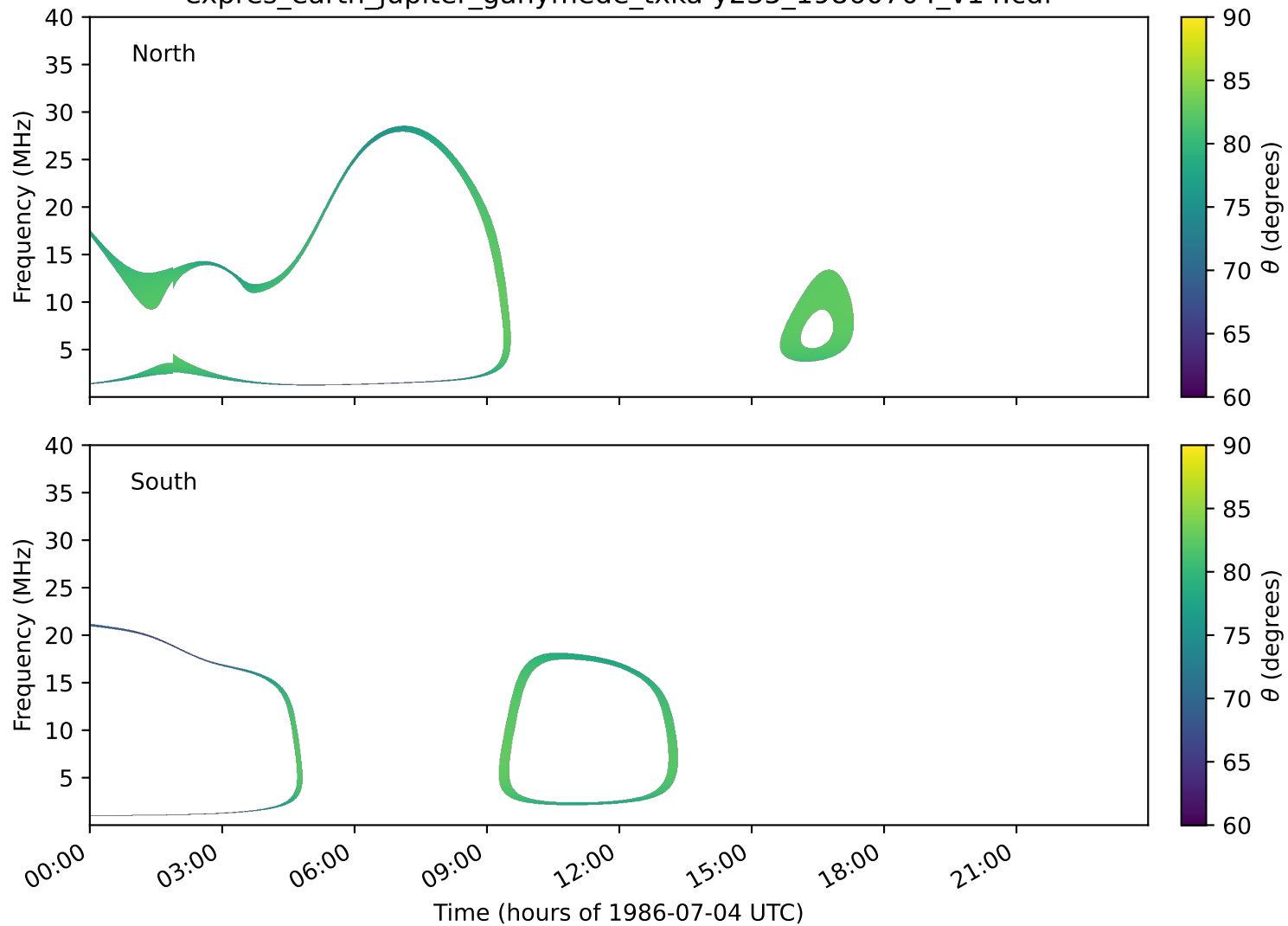
expres_earth_jupiter_ganymede_txka-y235_19860704_v14.cdf
