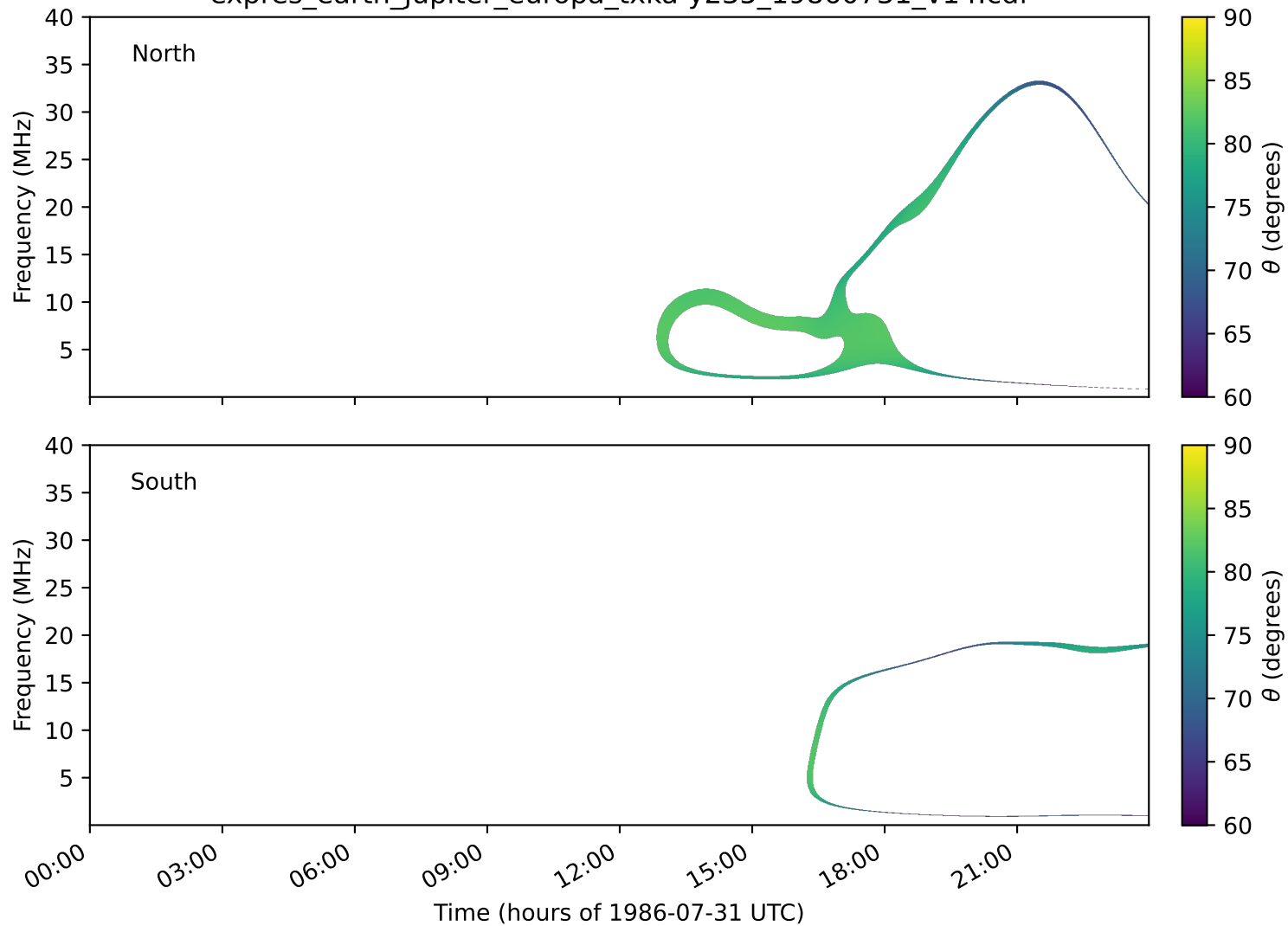
expres_earth_jupiter_europa_txka-y235_19860731_v14.cdf
