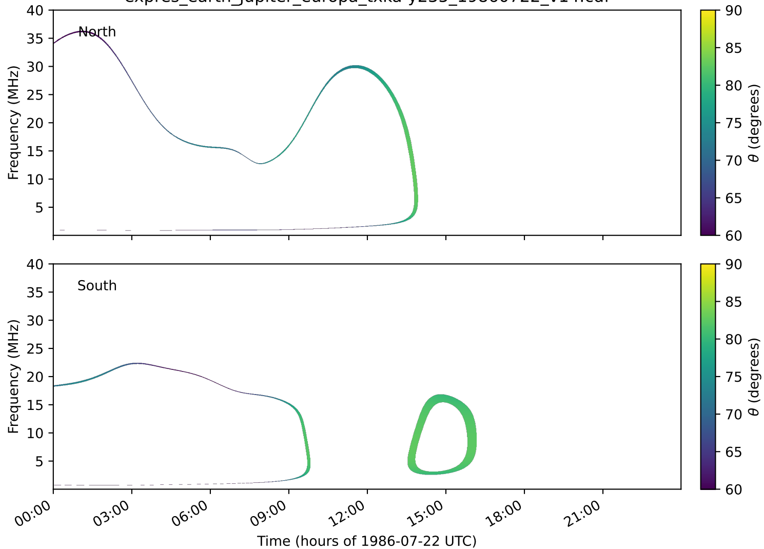
expres_earth_jupiter_europa_txka-y235_19860722_v14.cdf
