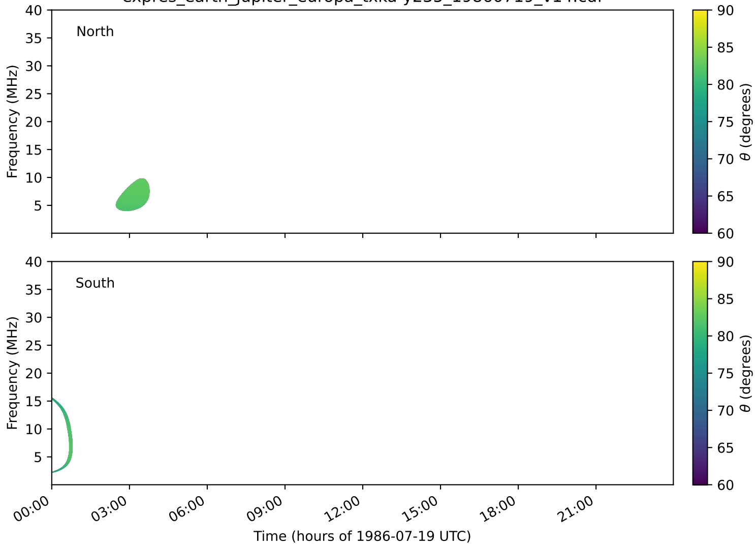
expres_earth_jupiter_europa_txka-y235_19860719_v14.cdf
