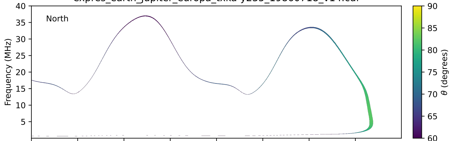
expres_earth_jupiter_europa_txka-y235_19860718_v14.cdf
