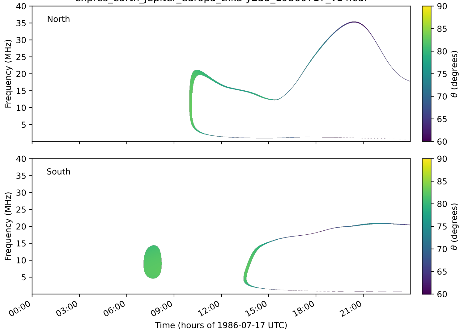
expres_earth_jupiter_europa_txka-y235_19860717_v14.cdf
