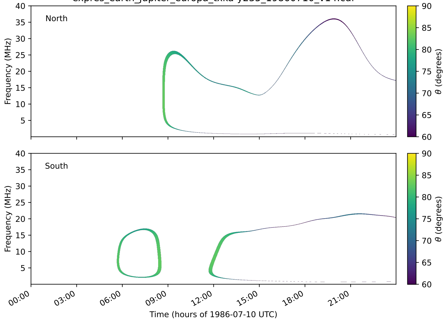
expres_earth_jupiter_europa_txka-y235_19860710_v14.cdf
