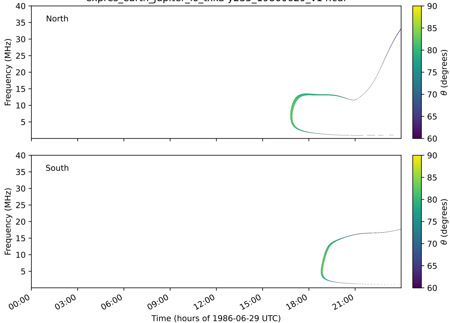
expres_earth_jupiter_io_txka-y235_19860629_v14.cdf
