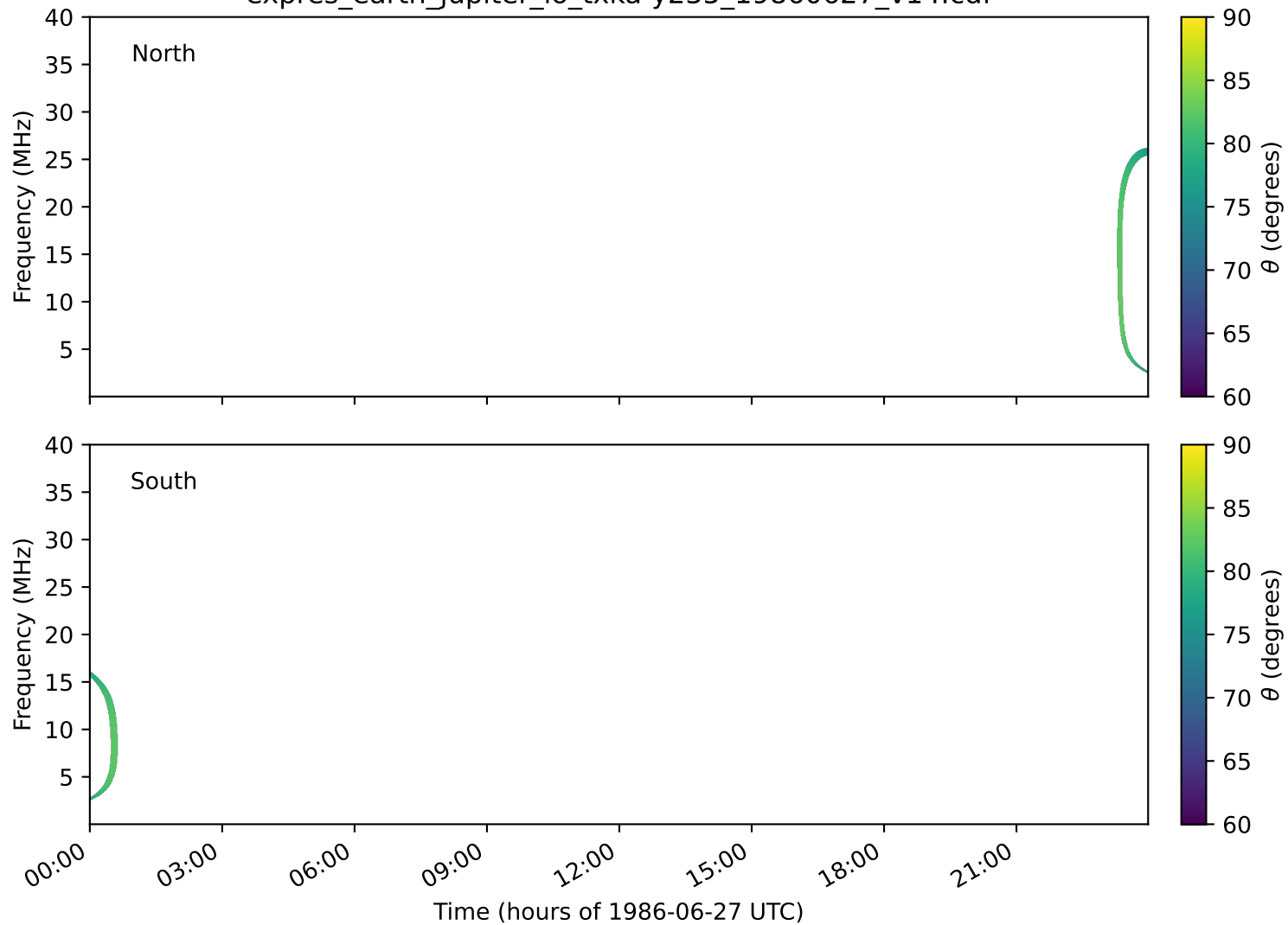
expres_earth_jupiter_io_txka-y235_19860627_v14.cdf
