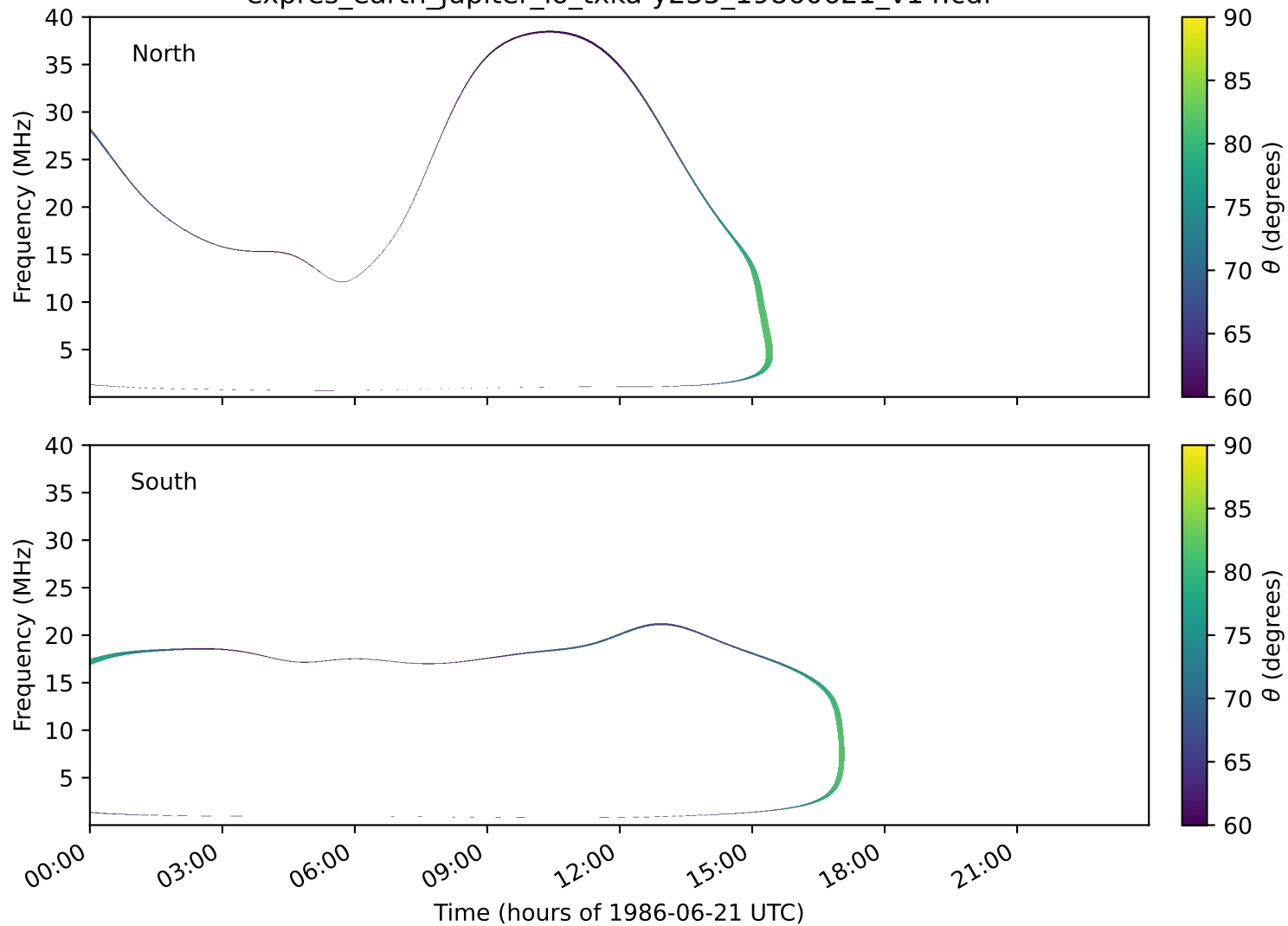
expres_earth_jupiter_io_txka-y235_19860621_v14.cdf
