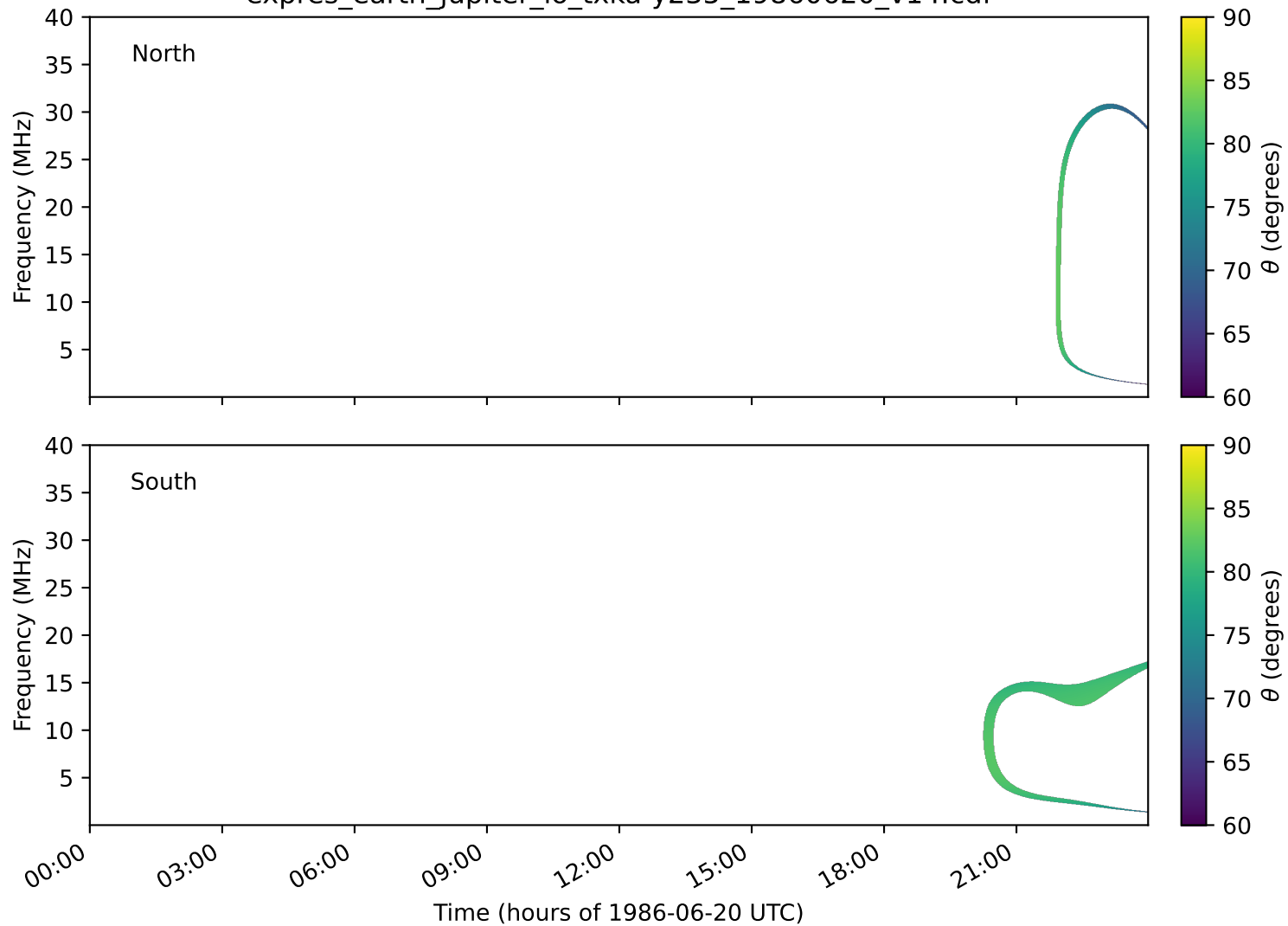
expres_earth_jupiter_io_txka-y235_19860620_v14.cdf
