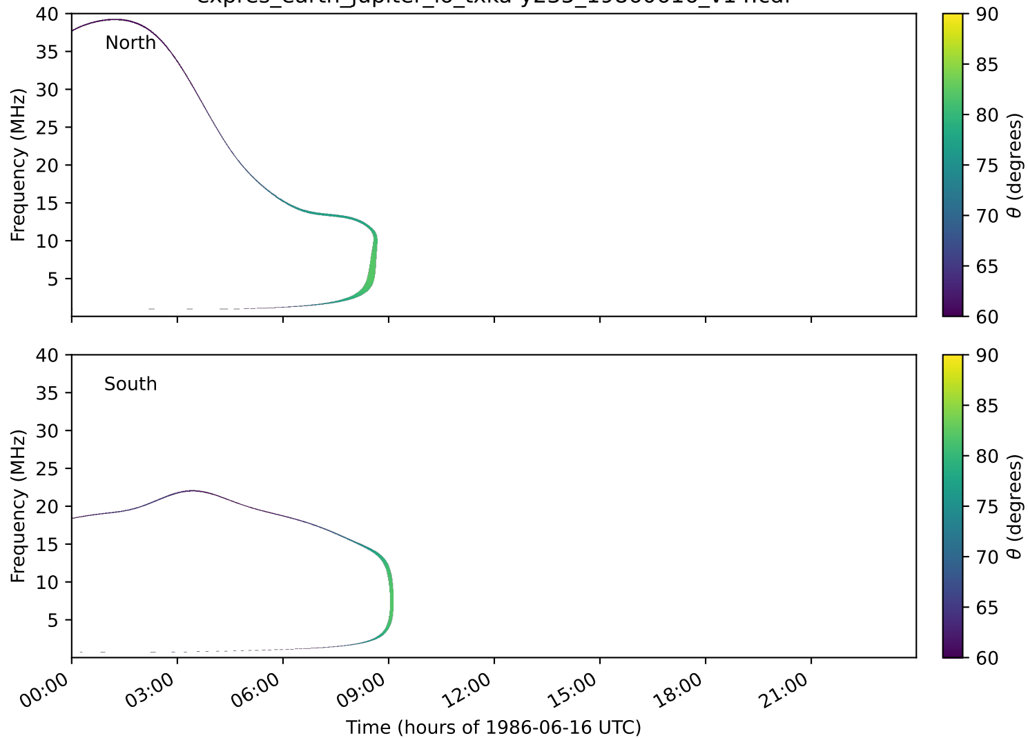
expres_earth_jupiter_io_txka-y235_19860616_v14.cdf
