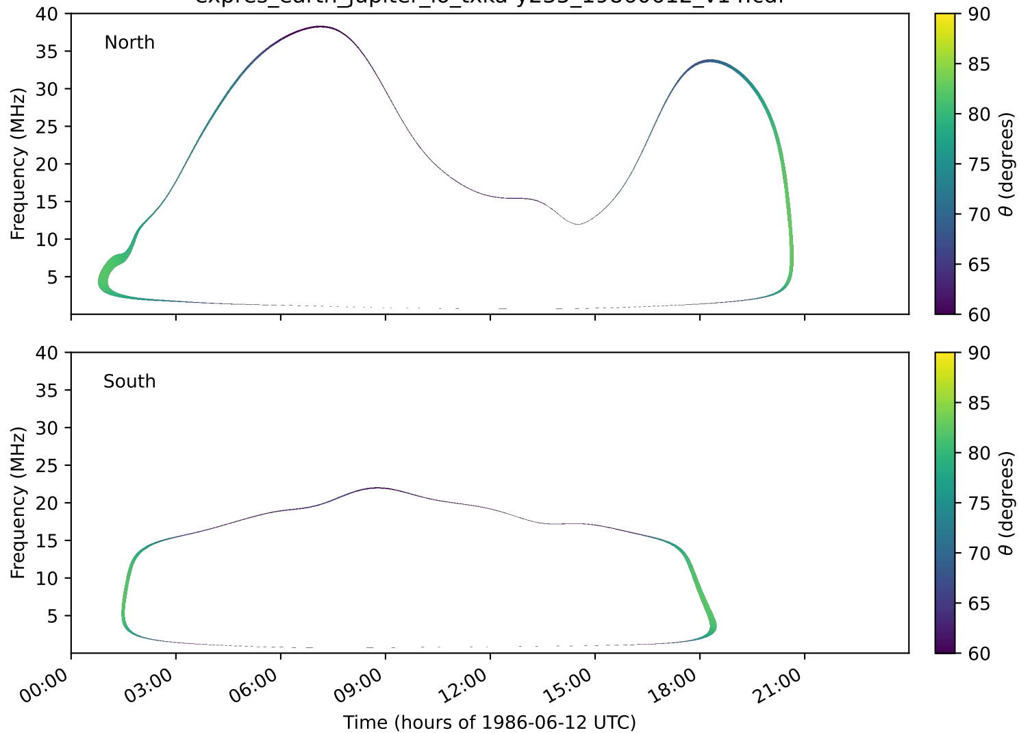
expres_earth_jupiter_io_txka-y235_19860612_v14.cdf
