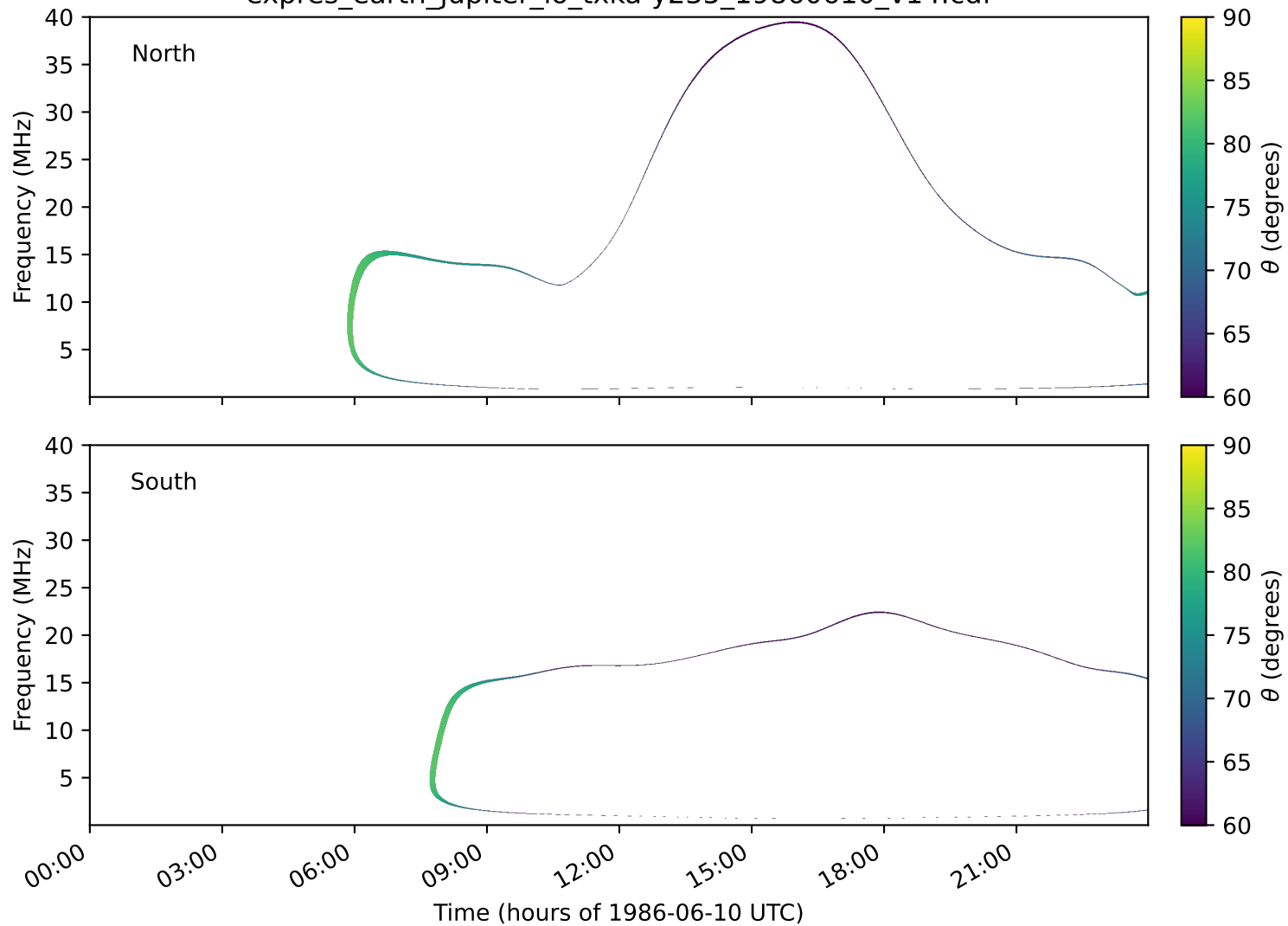
expres_earth_jupiter_io_txka-y235_19860610_v14.cdf
