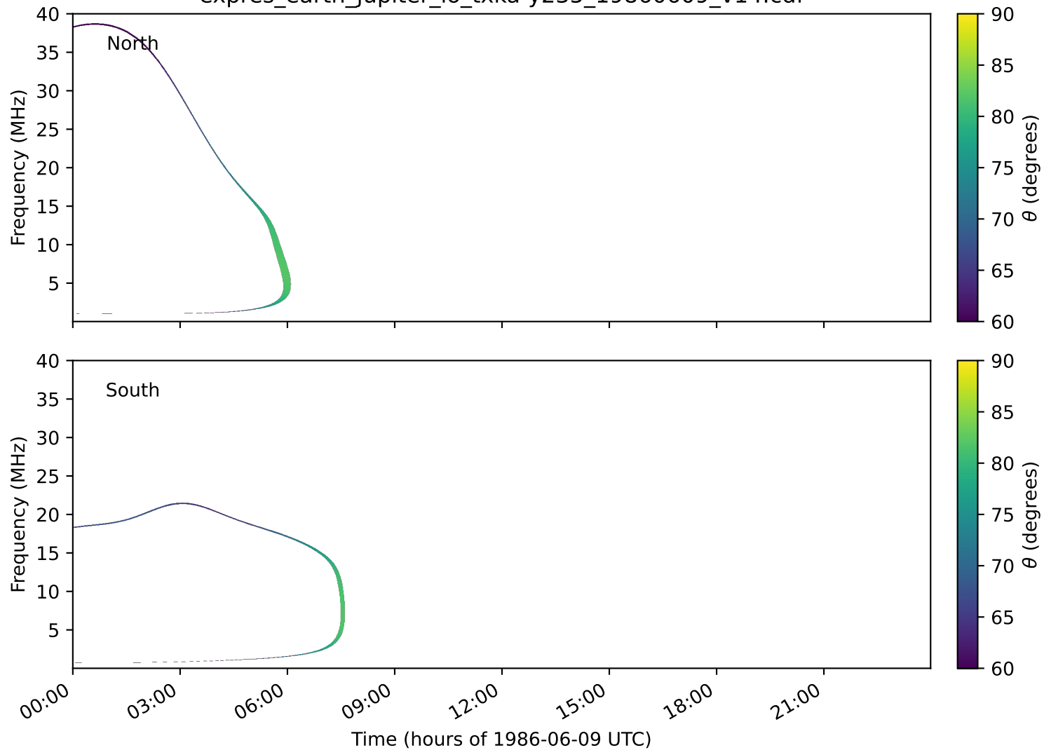
expres_earth_jupiter_io_txka-y235_19860609_v14.cdf
