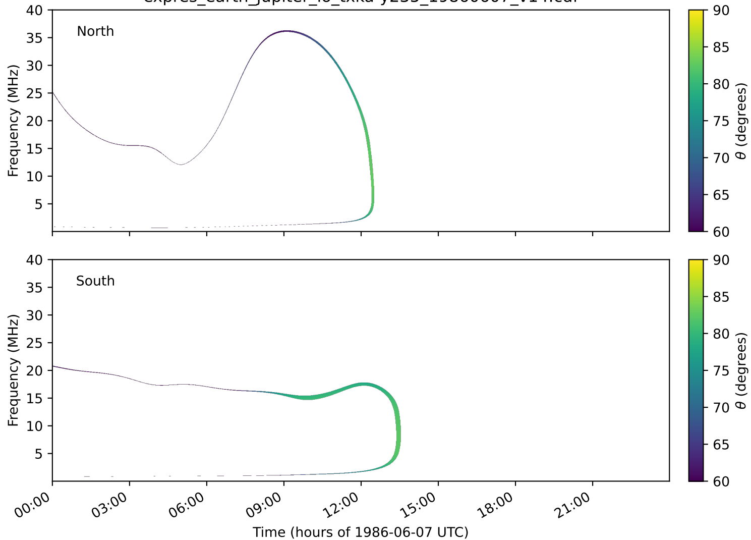
expres_earth_jupiter_io_txka-y235_19860607_v14.cdf
